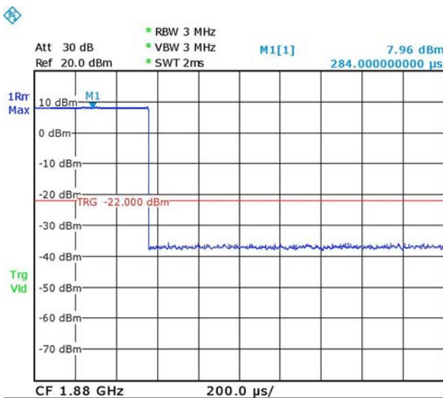
GSM Signal
