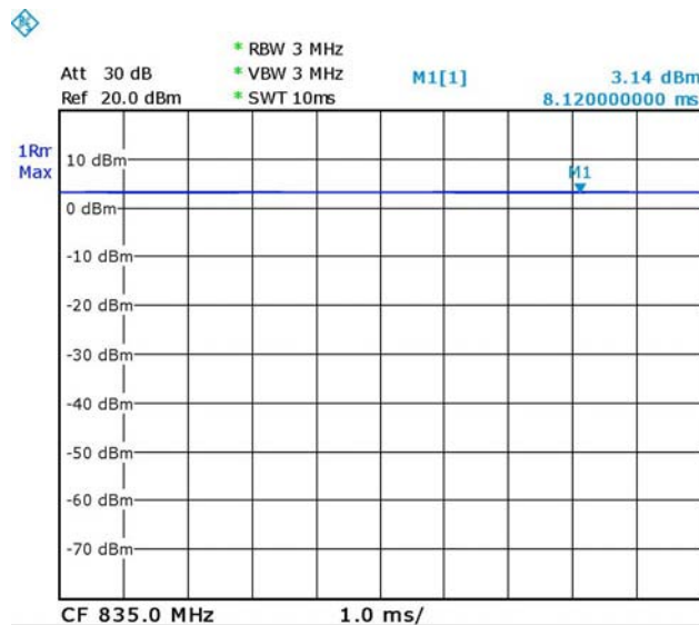
CW Signal
