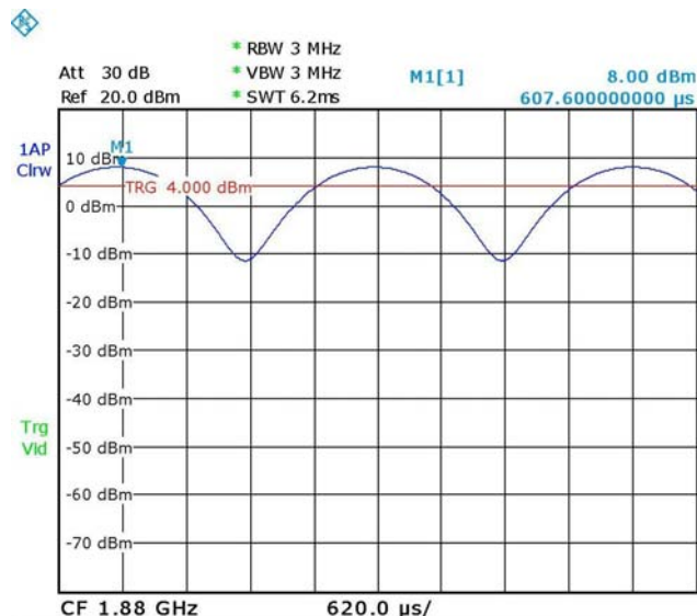
AM80%
