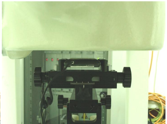
Bottom of the DUT with Phantom 1.5 cm Gap _Sample A
