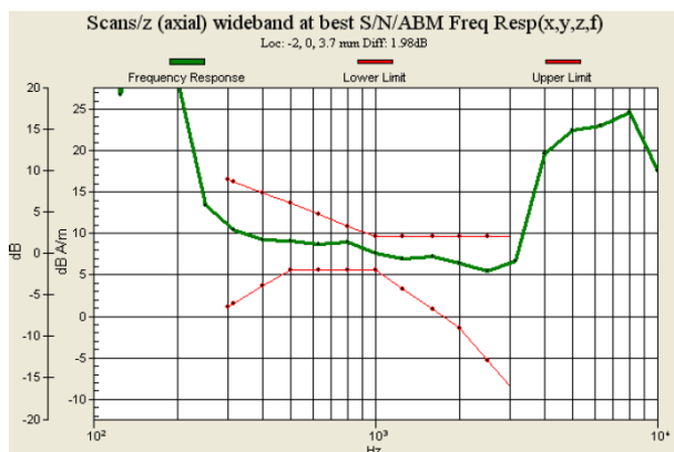
Fig. 9.3 GSM850 Ch251_Sample 1 with Battery 1_Slide Off
