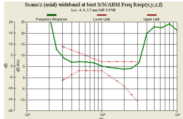
Fig. 9.14 WCDMA Band IV Ch1413_Sample 1 with Battery 1_Slide Off
