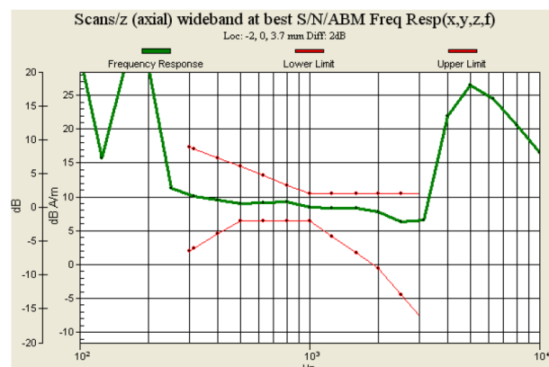
Fig. 9.6 GSM850 Ch189_Sample 2 with Battery 3_Slide Off
