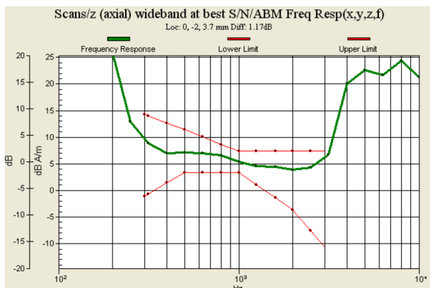
Fig. 9.17 WCDMA Band IV Ch1413_Sample 1 with Battery 1_Slide Right
