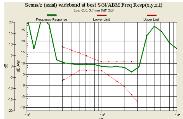
Fig. 9.12 GSM1900 Ch661_Sample 2 with Battery 3_Slide Off
