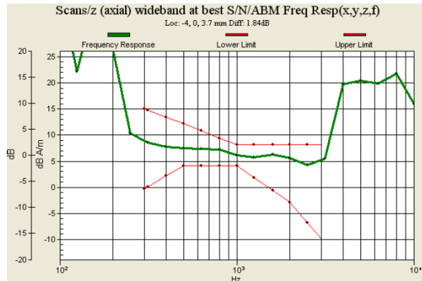
Fig. 9.7 GSM1900 Ch512_Sample 1 with Battery 1_Slide Off
