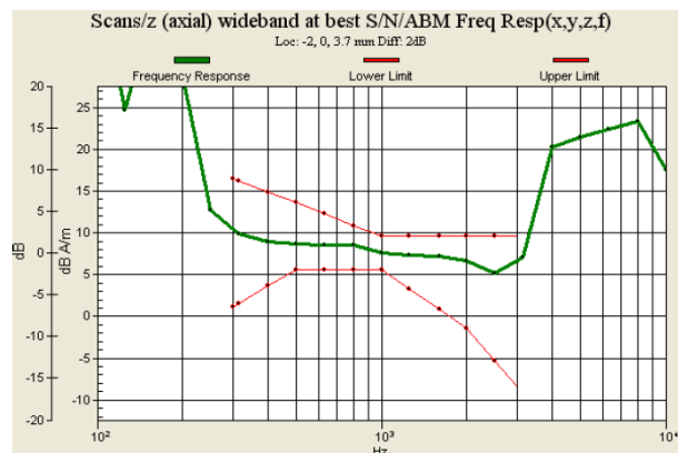
Fig. 9.4 GSM850 Ch189_Sample 2 with Battery 2_Slide Off
