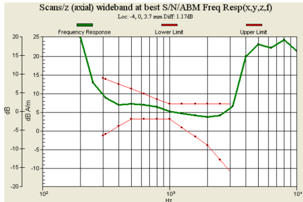
Fig. 9.13 WCDMA Band IV Ch1312_Sample 1 with Battery 1_Slide Off
