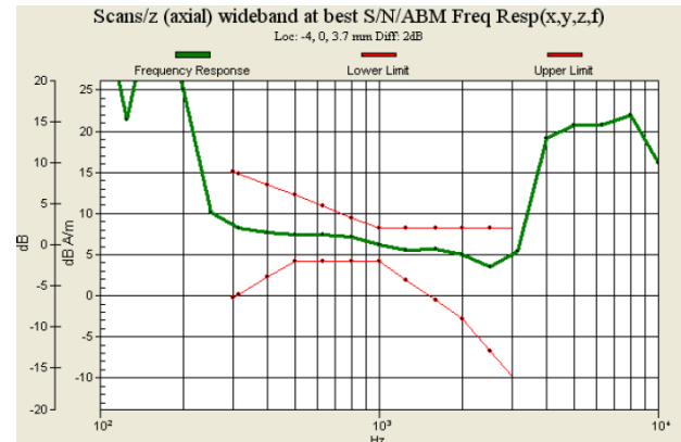
Fig. 9.8 GSM1900 Ch661_Sample 1 with Battery 1_Slide Off
