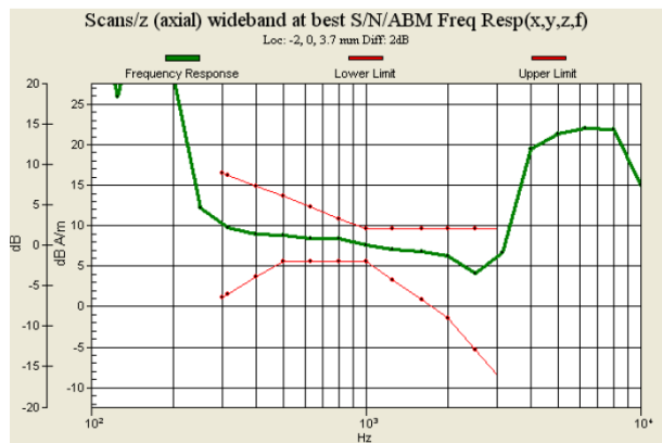
Fig. 9.11 GSM1900 Ch661_Sample 2 with Battery 2_Slide Right
