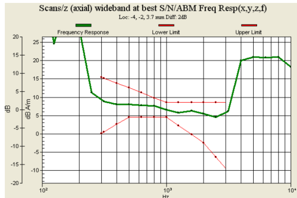
Fig. 9.9 GSM1900 Ch810_Sample 1 with Battery 1_Slide Off
