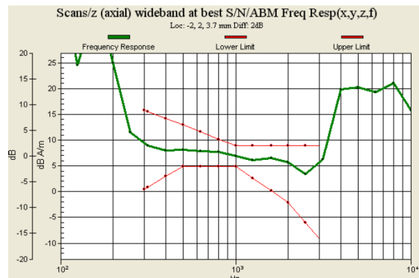
Fig. 9.2 GSM850 Ch189_Sample 1 with Battery 1_Slide Off
