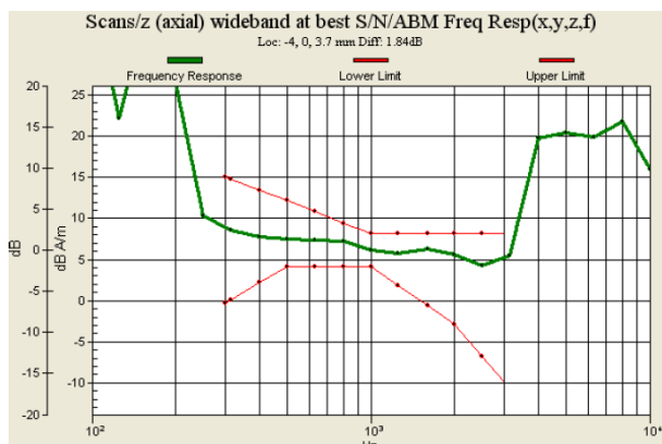
Fig. 9.5 GSM850 Ch189_Sample 2 with Battery 2_Slide Right
