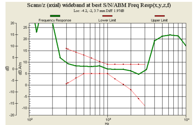
Fig. 9.10 GSM1900 Ch661_Sample 2 with Battery 2_Slide Off
