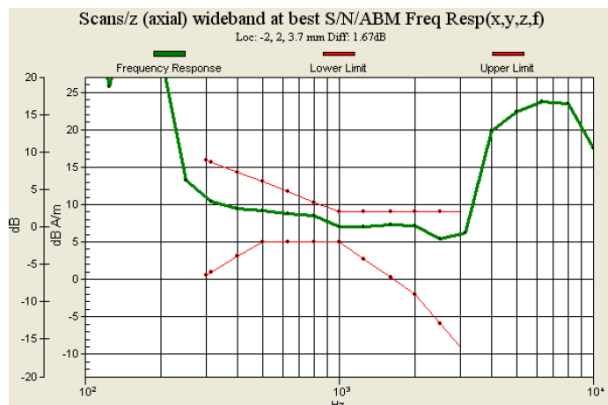
Fig. 9.1 GSM850 Ch128_Sample 1 with Battery 1_Slide Off
