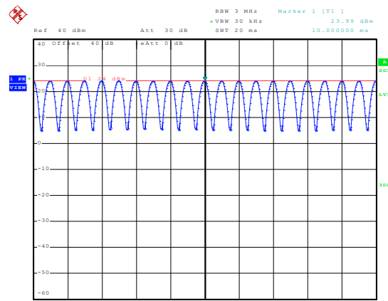
835MHz - 80% AM
