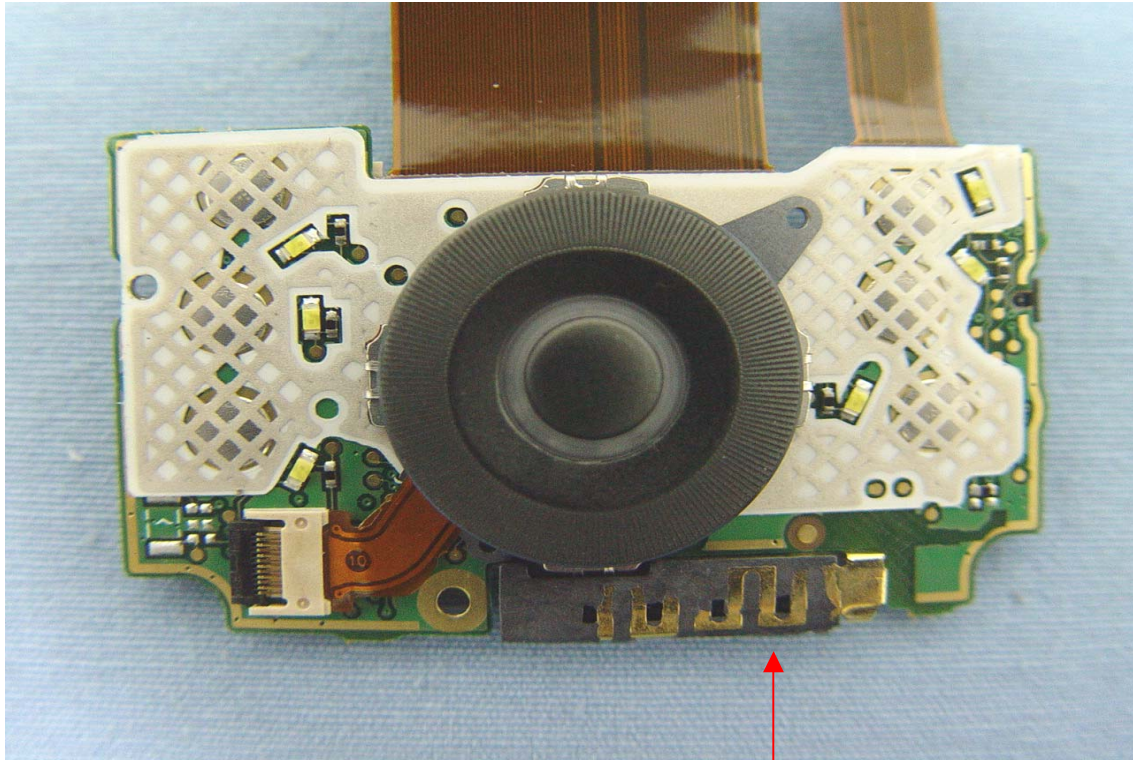
WLAN Antenna
