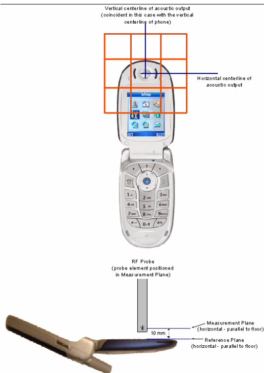
Figure 13: WD near-field emission test setup
