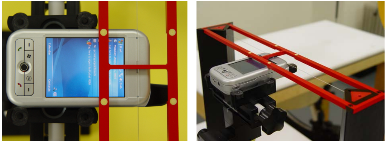
CDMA Cellular Band Duty cycle:100%
