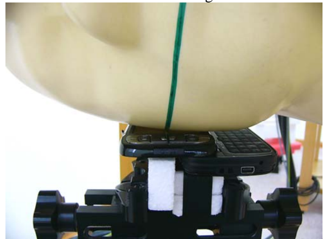
Fig.4 Right Head at Slider-on Section / Cheek-Touch Position
