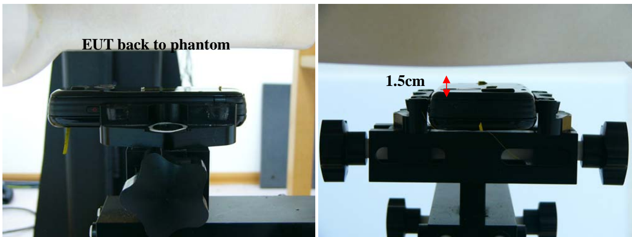
Fig.14 Body worn- EUT back to flat phantom and distance between flat phantom and mobile phone is 1.5 cm
