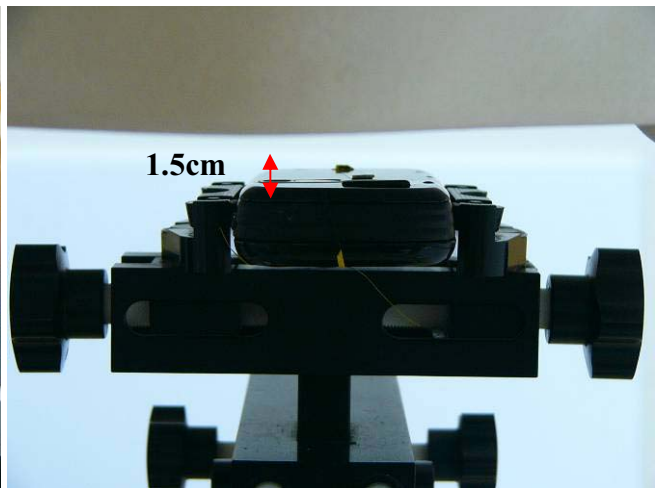
Fig.14 Body worn- EUT back to flat phantom and distance between flat phantom and mobile phone is 1.5 cm
