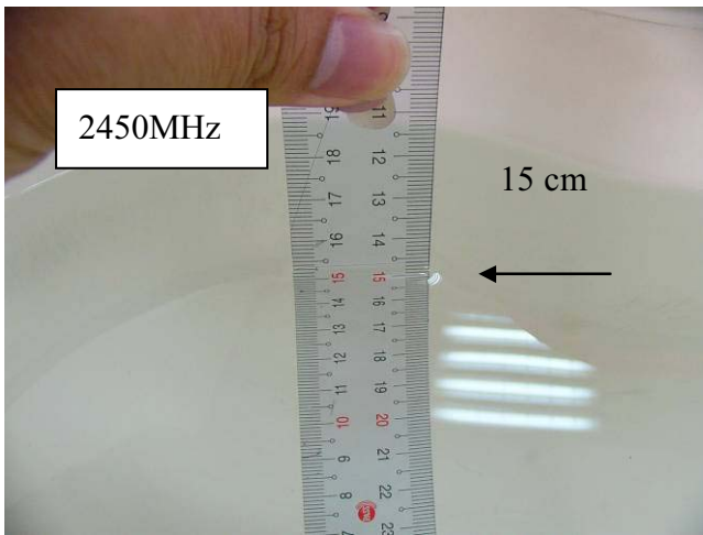
Fig.2.3 Photograph of the Tissue Simulant Fluid liquid depth 15cm for Right-head Side
