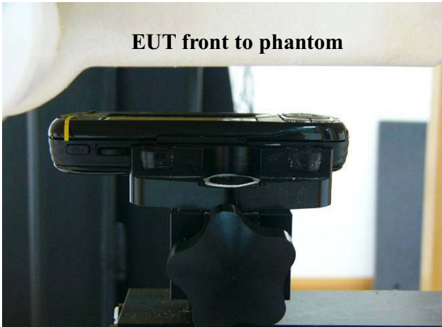
Fig.13 Body worn- EUT front to flat phantom and distance between flat phantom and mobile phone is 1.5 cm
