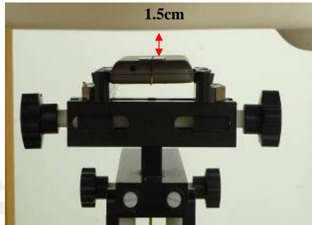
Fig.8 Body worn- EUT back to flat phantom and distance between flat phantom and mobile phone is 1.5 cm
