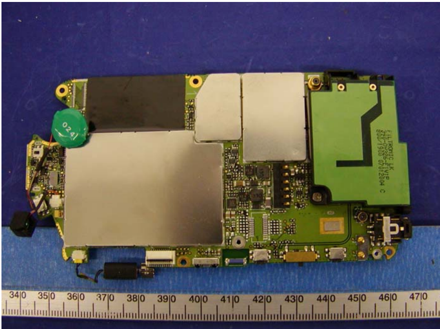
PH20A3 EUT – Component View with Shielding
