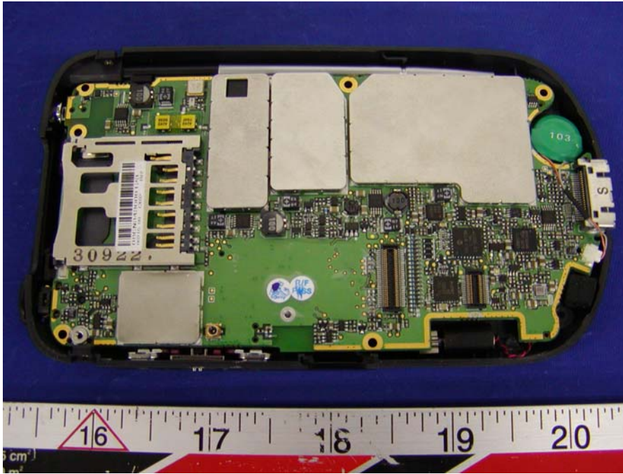
PH20A2 Chassis – Cover off View
