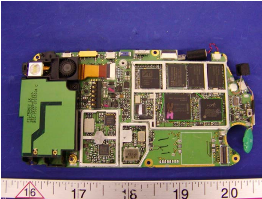
PH20A2 EUT – Component View without Shielding
