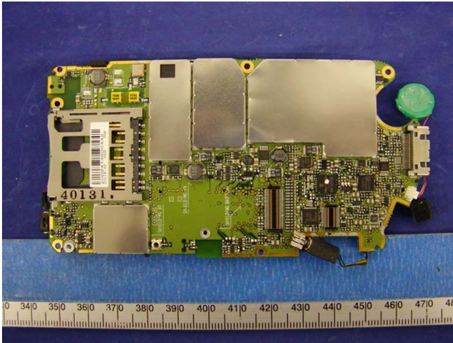
PH20A3 EUT – Solder View with Shielding
