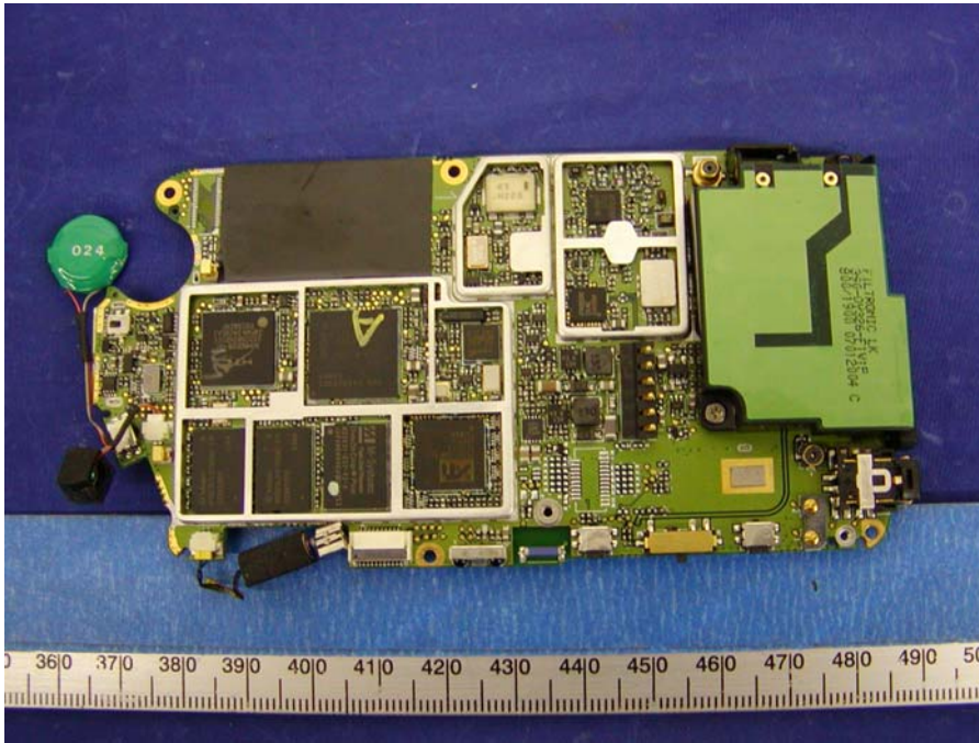
PH20A3 EUT – Component View without Shielding
