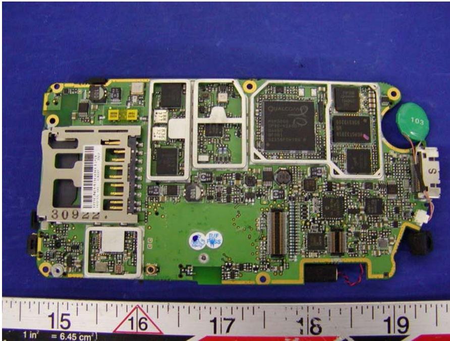
PH20A2 EUT – Solder View without Shield
