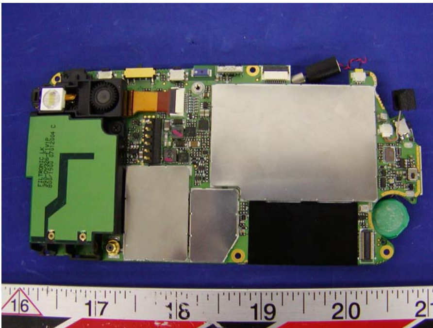
PH20A2 EUT – Component View with Shielding
