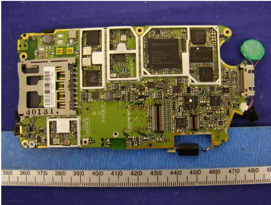
PH20A3 EUT – Solder View without Shield
