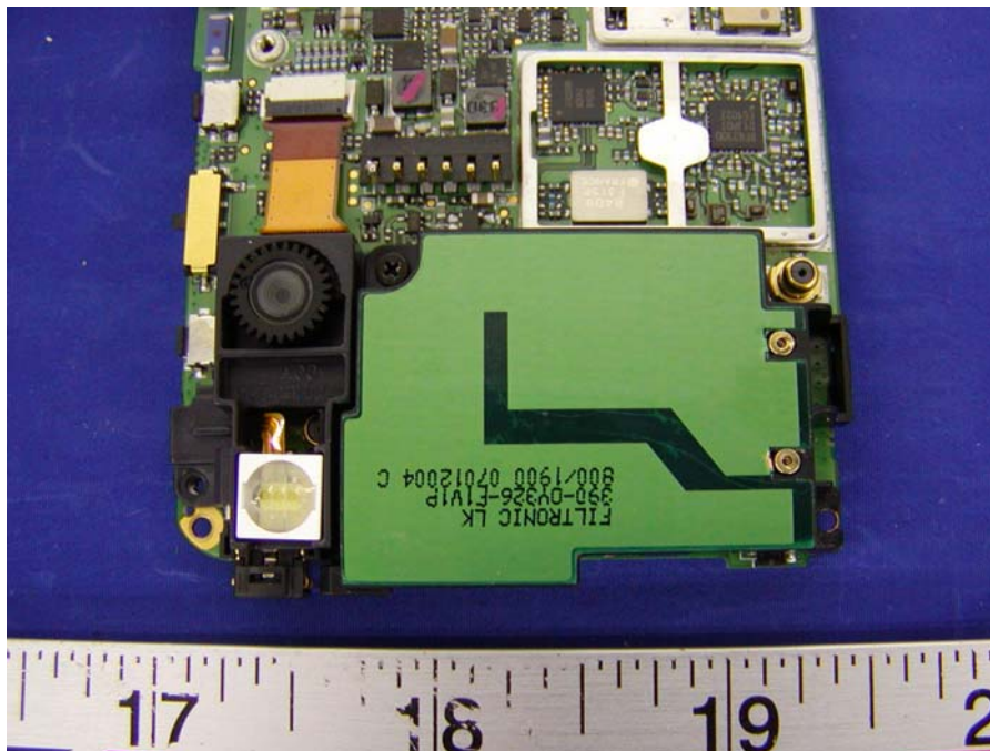
PH20A2 EUT – Antenna View
