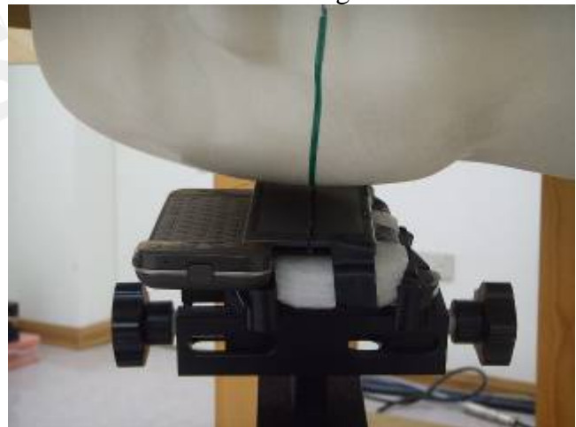
Fig.6 Right Head at Slider-on Section / Ear-Tilt Position(15°)
