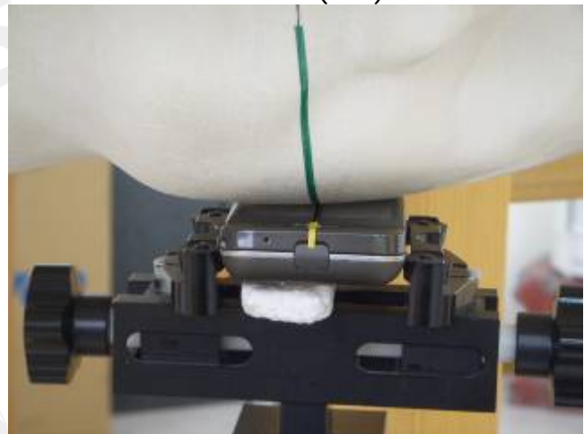
Fig.7 Left Head at Slider-off Section / Cheek-Touch Position
