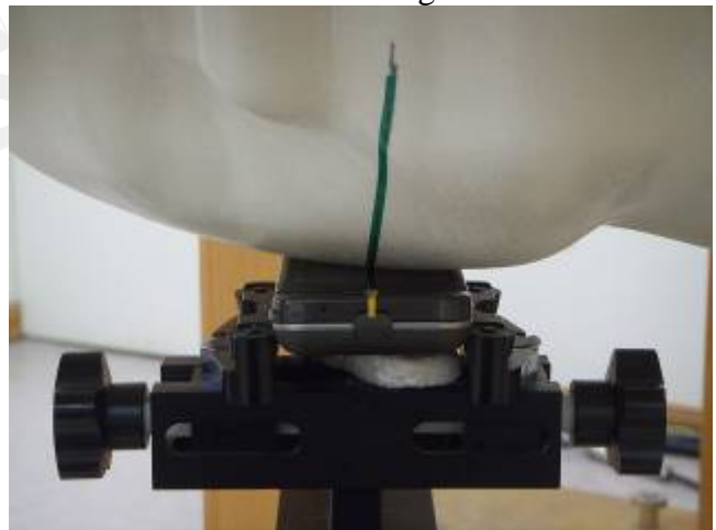
Fig.3 Right Head at Slider-off Section / Cheek-Touch Position
