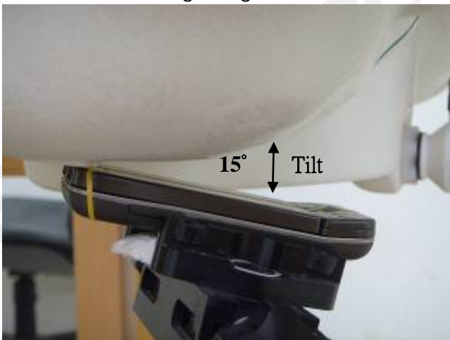
Fig.5 Right Head at Slider-off Section / Ear-Tilt Position(15°)
