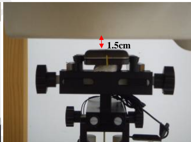
Fig.13 Body worn- EUT back to flat phantom and distance between flat phantom and mobile phone is 1.5 cm_repeated with handset
