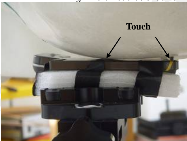
Fig.8 Left Head at Slider-on Section / Cheek-Touch Position
