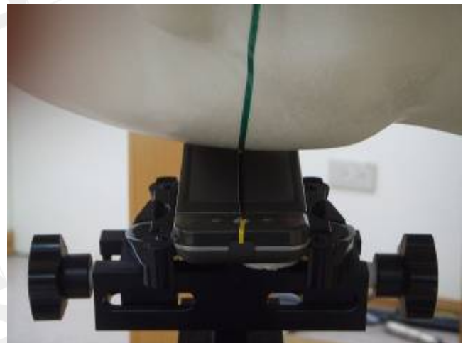
Fig.5 Right Head at Slider-off Section / Ear-Tilt Position(15°)
