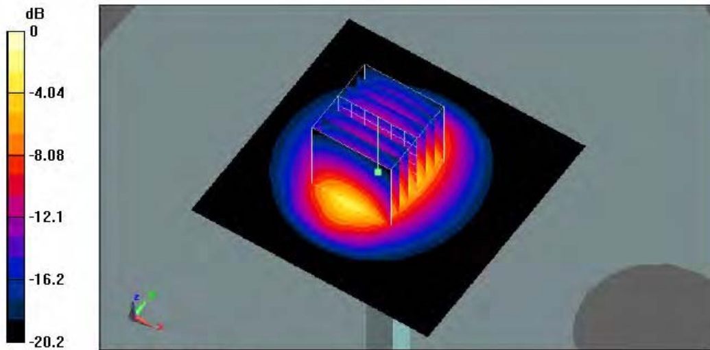
0 dB = 6.09mW/g
