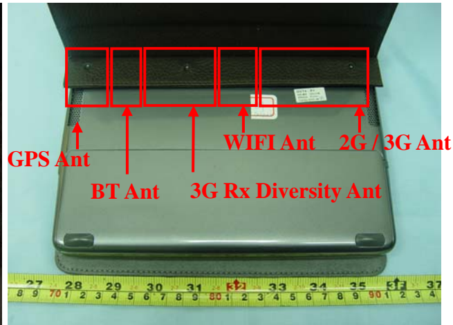
The exterior case of EUT relates to all of antennas positions
