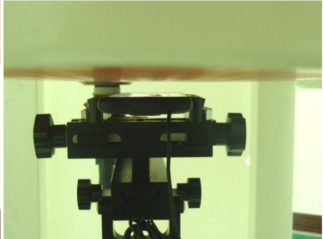
Front Face of the DUT with Phantom 1.0 cm Gap for DUT with Earphone
