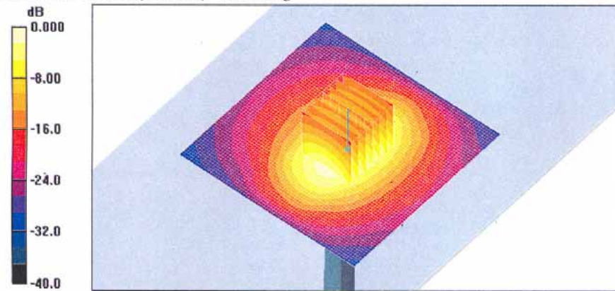
0 dB = 11.1 mW/g
