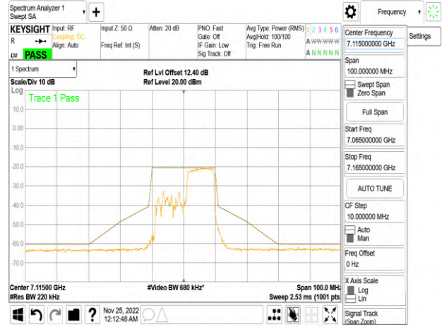
802.11ax_20MHz_Chain1_7115MHz_RU106_54
