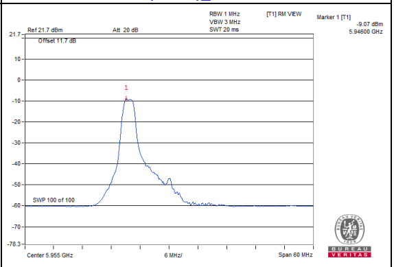
802.11ax (RU106)_Chain 1 / CH1
