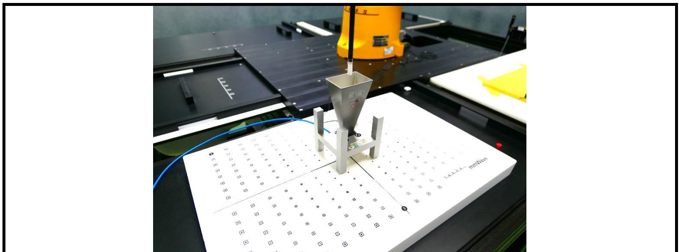
Fig-3.3 System Verification Setup
