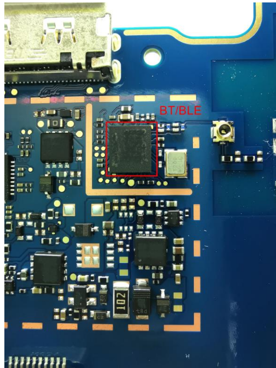
Internal View of EUT – 4
