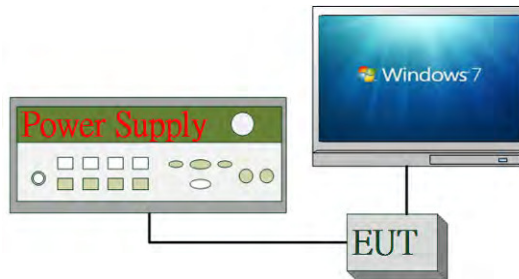
Fig. 2-3 Conduction Emission Configuration
