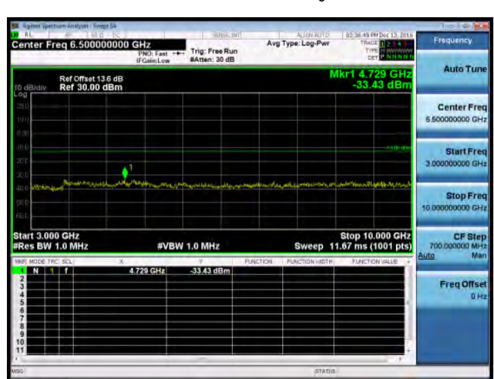
3GHz~10GHz_Band5_5MHz_QPSK_1_0_HighCH20625-846.5
