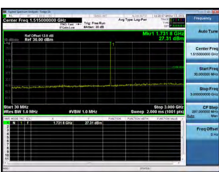
30MHz~3GHz_Band4_5MHz_QPSK_1_0_MidCH20175-1732.5
