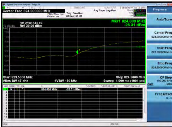
Band Edge_HSUPA_B5_LowCH4132-826.4
