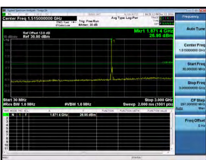
30MHz~3GHz_Band2_20MHz_QPSK_1_0_MidCH18900-1880
