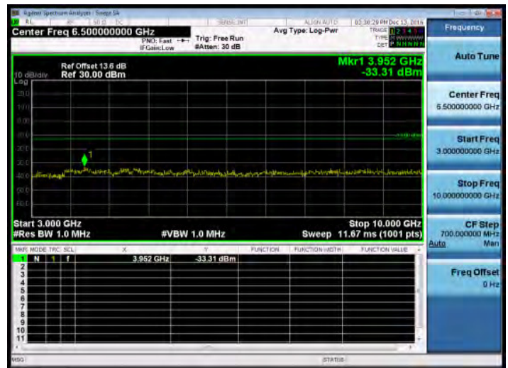
3GHz~10GHz_Band5_10MHz_QPSK_1_0_MidCH20525-836.5
