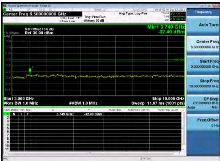
3GHz~10GHz_Band12_10MHz_QPSK_1_0_LowCH23060-704
