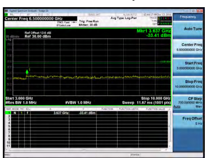
3GHz~10GHz_Band5_3MHz_QPSK_1_0_HighCH20635-847.5
