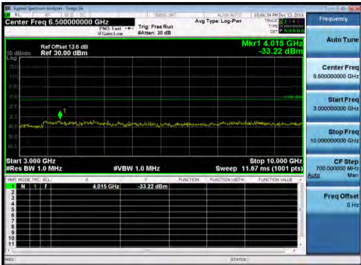
3GHz-10GHz_Band12_1.4MHz_QPSK_1_0_LowCH23017-699.7
