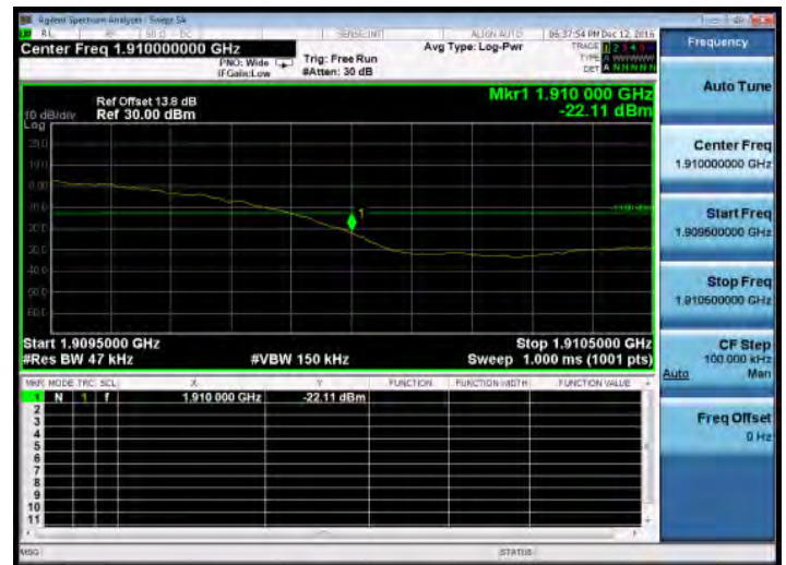
Band Edge_WCDMA_B2_HighCH9538-1907.6
