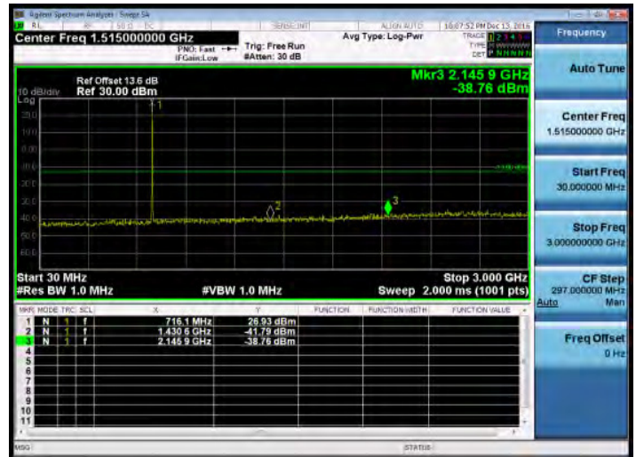
30MHz-3GHz_Band12_1.4MHz_QPSK_1_0_HighCH23173-715.3
