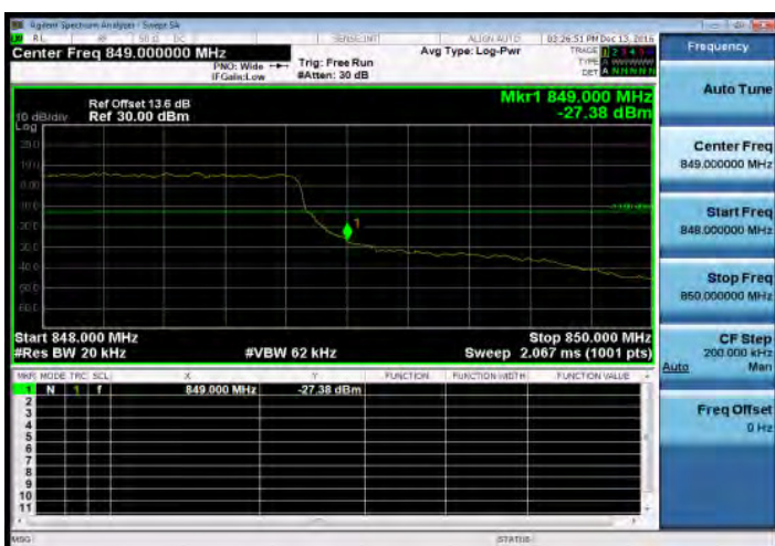
Band Edge_Band5_1.4MHz_QPSK_6_0_HighCH20643-848.3
