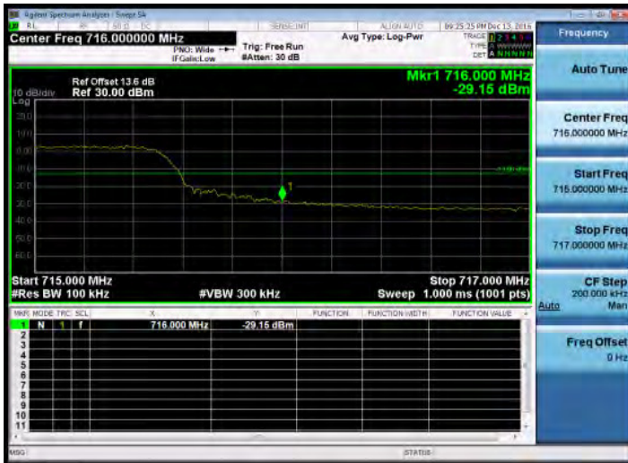
Band Edge_Band12_10MHz_QPSK_50_0_HighCH23130-711
