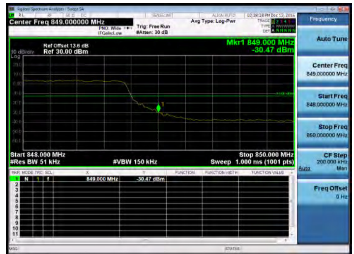
Band Edge_Band5_5MHz_QPSK_25_0_HighCH20625-846.5
