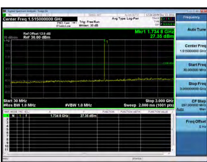
30MHz-3GHz_Band4_1.4MHz_QPSK_1_0_MidCH20175-1732.5
