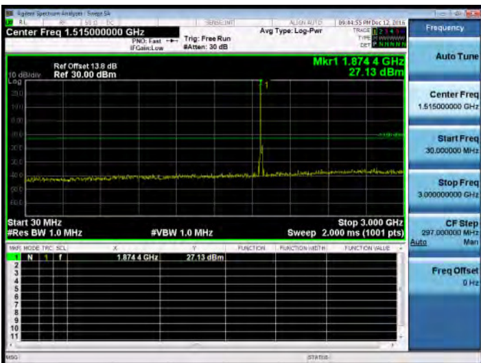
30MHz~3GHz_Band2_15MHz_QPSK_1_0_MidCH18900-1880
