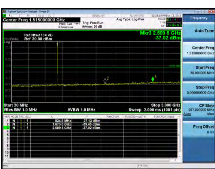
30MHz~3GHz_Band5_5MHz_QPSK_1_0_MidCH20525-836.5
