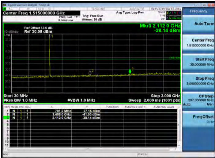
30MHz~3GHz_Band12_10MHz_QPSK_1_0_LowCH23060-704
