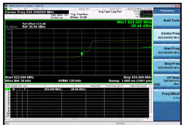
Band Edge_Band5_3MHz_QPSK_15_0_LowCH20415-825.5
