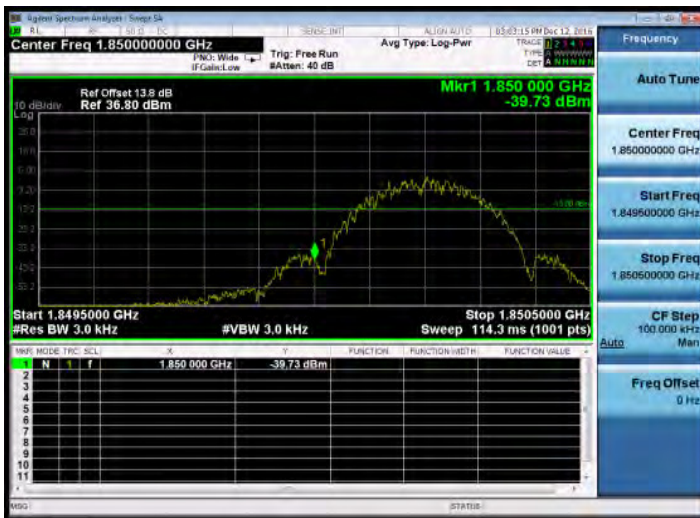
Band Edge_EDGE_1900MHz_LowCH512-1850.2
