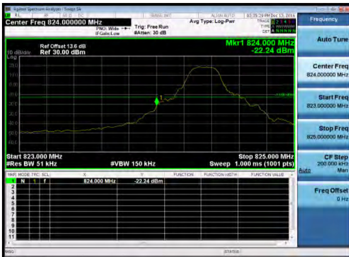
Band Edge_Band5_5MHz_QPSK_1_0_LowCH20425-826.5
