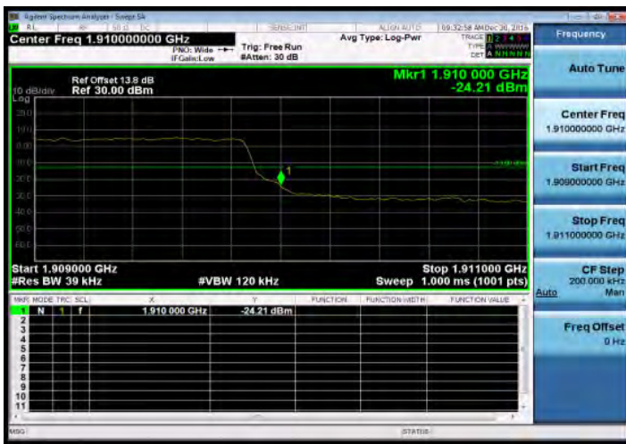
Band Edge_Band2_3MHz_QPSK_15_0_HighCH19185-1908.5
