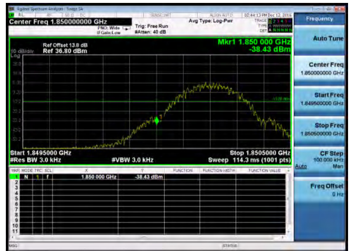
Band Edge_GPRS_1900MHz_LowCH512-1850.2
