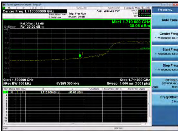
Band Edge_Band4_10MHz_QPSK_50_0_LowCH20000-1715
