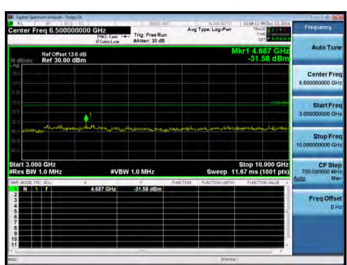
3GHz-10GHz_Band12_1.4MHz_QPSK_1_0_HighCH23173-715.3
