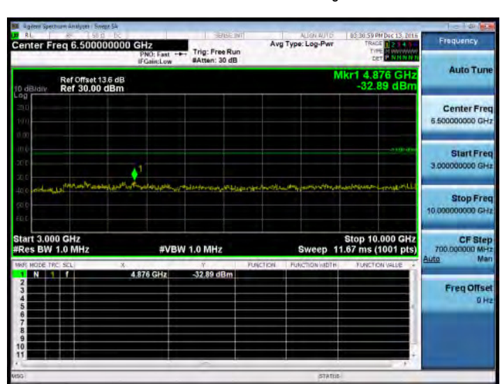
3GHz~10GHz_Band5_10MHz_QPSK_1_0_HighCH20600-844
