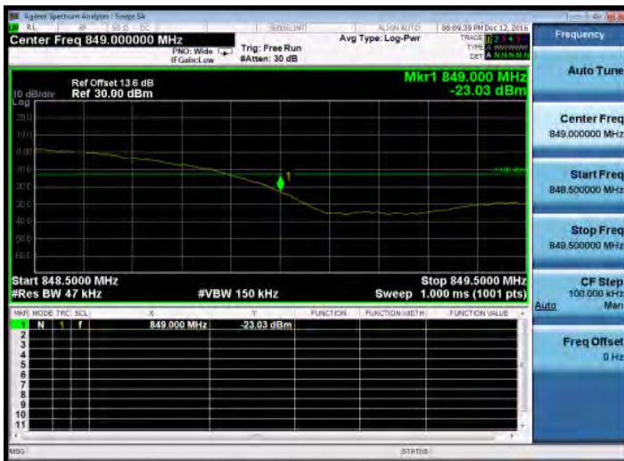
Band Edge_HSUPA_B5_HighCH4233-846.6
