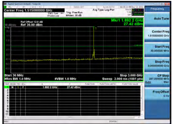
30MHz~3GHz_Band2_20MHz_QPSK_1_0_HighCH19100-1900
