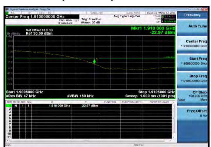
Band Edge_HSDPA_B2_HighCH9538-1907.6
