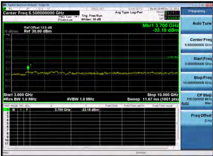
3GHz~10GHz_Band12_3MHz_QPSK_1_0_LowCH23025-700.5
