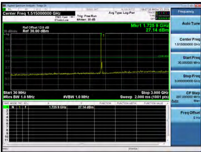
30MHz~3GHz_Band4_20MHz_QPSK_1_0_MidCH20175-1732.5
