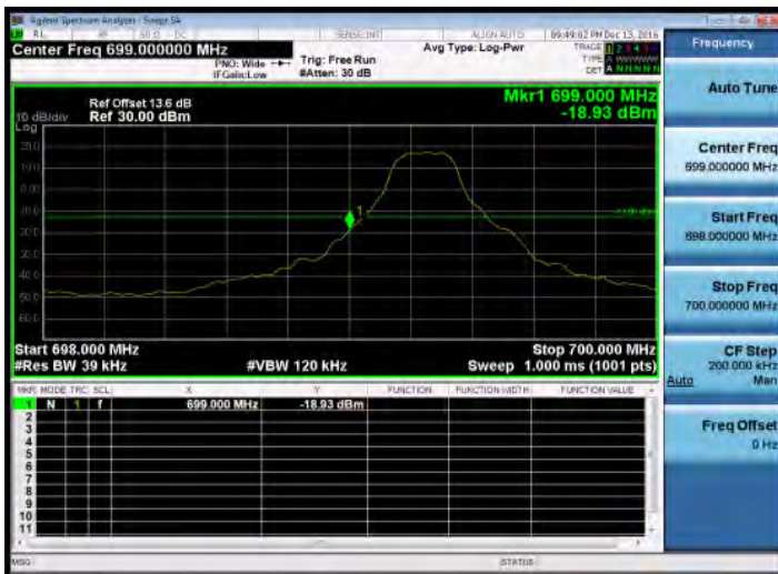
Band Edge_Band12_3MHz_QPSK_1_0_LowCH23025-700.5
