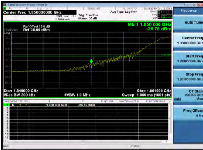
Band Edge_Band2_20MHz_QPSK_1_0_LowCH18700-1860
