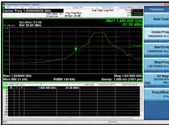
Band Edge_Band2_5MHz_QPSK_1_0_LowCH18625-1852.5
