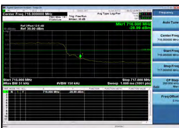
Band Edge_Band12_5MHz_QPSK_25_0_HighCH23155-713.5
