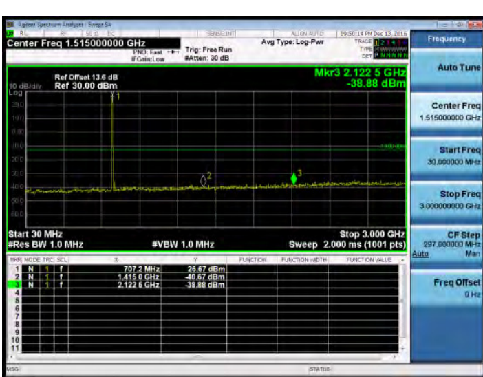
30MHz~3GHz_Band12_3MHz_QPSK_1_0_MidCH23095-707.5
