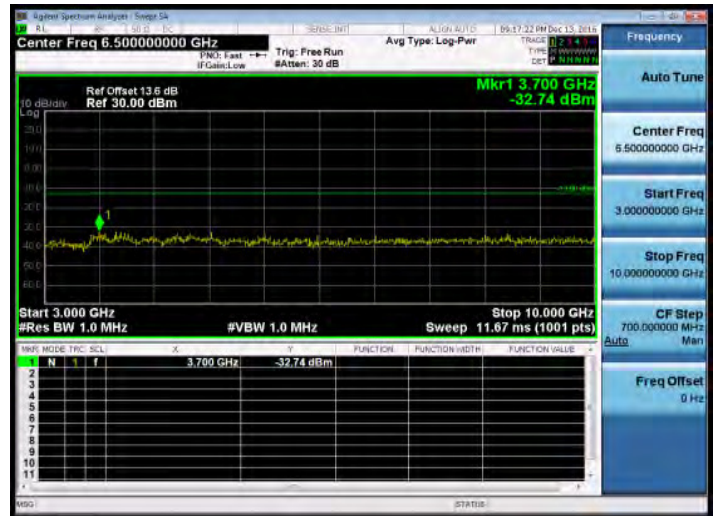
3GHz~10GHz_Band12_10MHz_QPSK_1_0_MidCH23095-707.5
