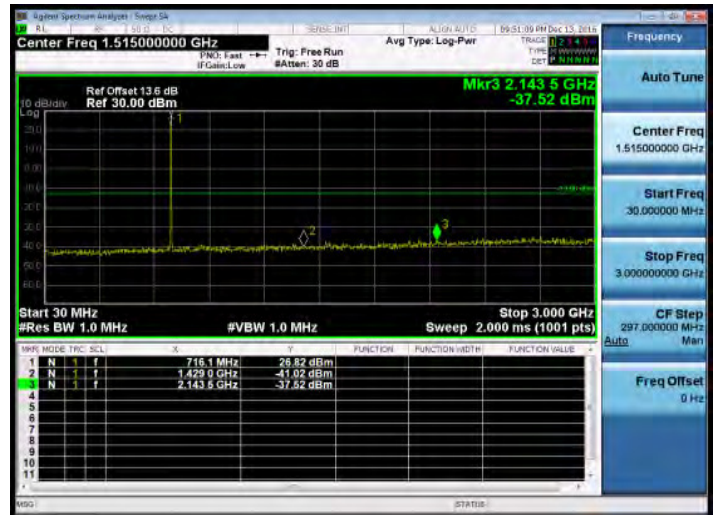
30MHz~3GHz_Band12_3MHz_QPSK_1_0_HighCH23165-714.5
