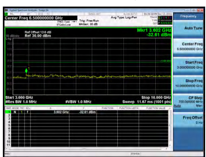
3GHz~10GHz_Band12_5MHz_QPSK_1_0_HighCH23155-713.5
