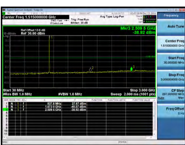
30MHz~3GHz_Band5_3MHz_QPSK_1_0_MidCH20525-836.5
