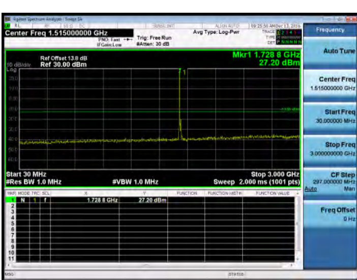
30MHz~3GHz_Band4_15MHz_QPSK_1_0_MidCH20175-1732.5
