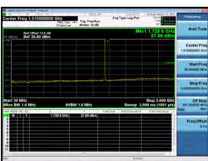
30MHz~3GHz_Band4_10MHz_QPSK_1_0_MidCH20175-1732.5
