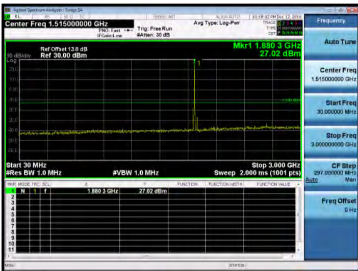
30MHz~3GHz_Band2_5MHz_QPSK_1_0_MidCH18900-1880
