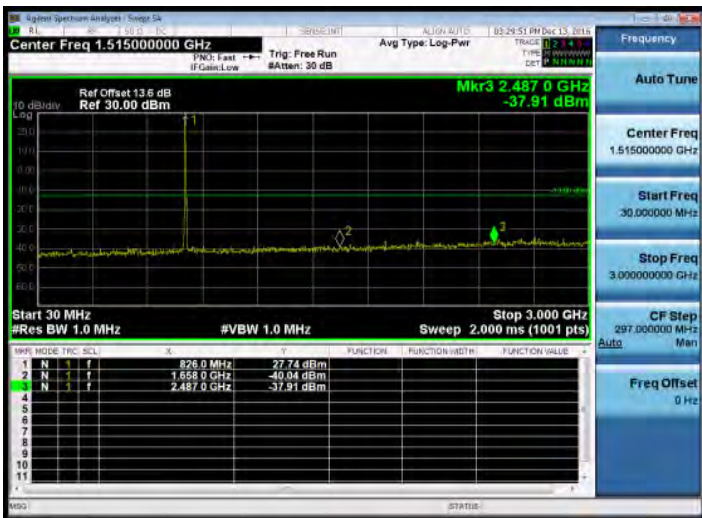
30MHz~3GHz_Band5_10MHz_QPSK_1_0_LowCH20450-829
