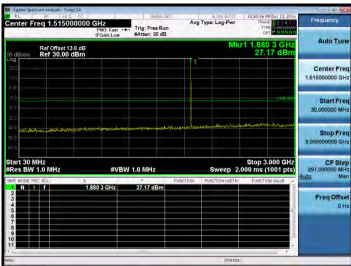
30MHz~3GHz_Band2_3MHz_QPSK_1_0_MidCH1890-1880
