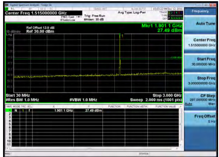
30MHz~3GHz_Band2_10MHz_QPSK_1_0_HighCH19150-1905
