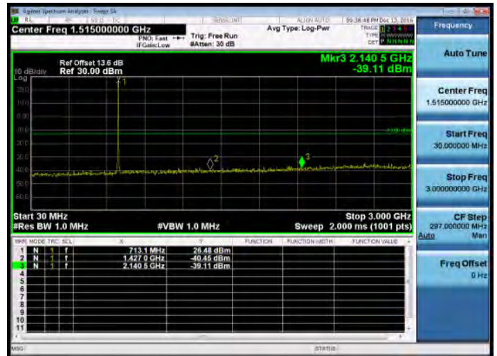
30MHz~3GHz_Band12_5MHz_QPSK_1_0_HighCH23155-713.5
