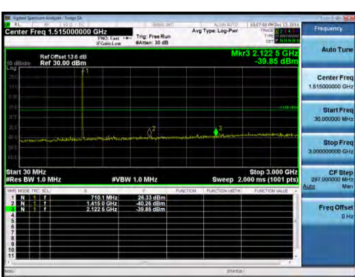
30MHz-3GHz_Band12_1.4MHz_QPSK_1_0_MidCH23095-707.5
