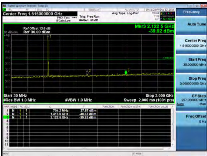
30MHz~3GHz_Band12_10MHz_QPSK_1_0_MidCH23095-707.5
