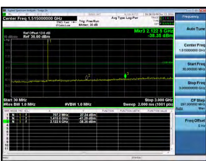
30MHz~3GHz_Band12_5MHz_QPSK_1_0_MidCH23095-707.5
