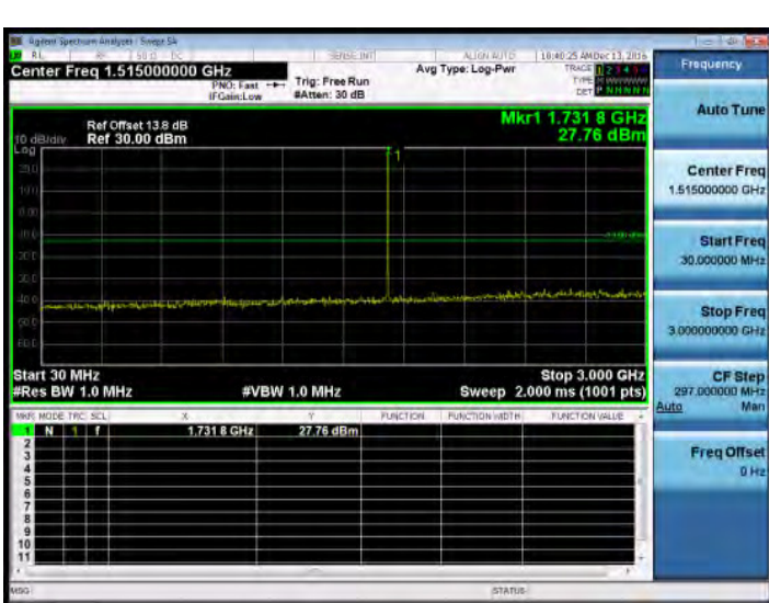
30MHz~3GHz_Band4_3MHz_QPSK_1_0_MidCH20175-1732.5
