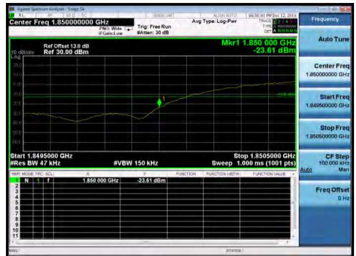
Band Edge_HSDPA_B2_LowCH9262-1852.4
