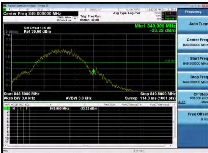
Band Edge_GSM_850MHz_HighCH251-848.8
