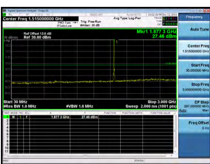
30MHz~3GHz_Band2_10MHz_QPSK_1_0_MidCH18900-1880
