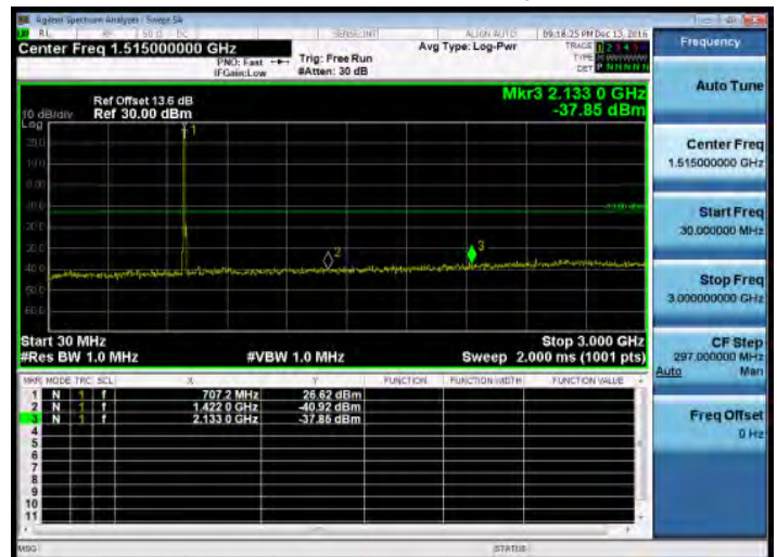
30MHz~3GHz_Band12_10MHz_QPSK_1_0_HighCH23130-711
