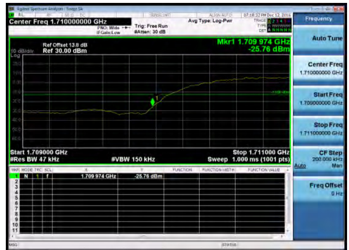
Band Edge_HSDPA_B4_LowCH1312-1712.4
