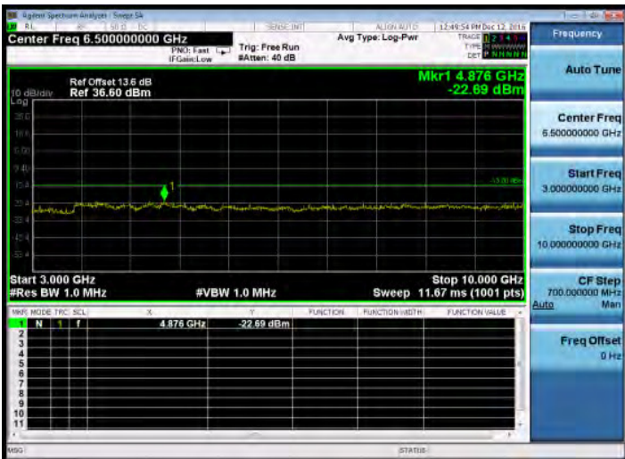
3GHz~10GHz_GSM_850MHz_LowCH128-824.2
