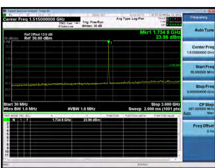
30MHz~3GHz_HSUPA_B4_MidCH1413-1732.6
