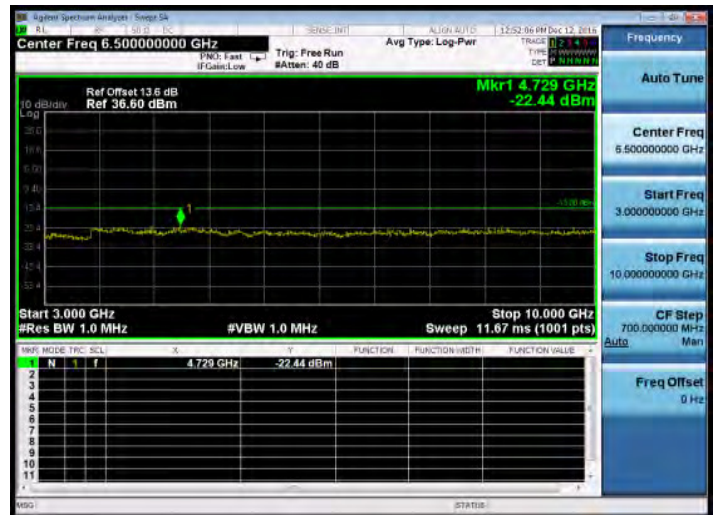
3GHz~10GHz_GSM_850MHz_MidCH190-836.6
