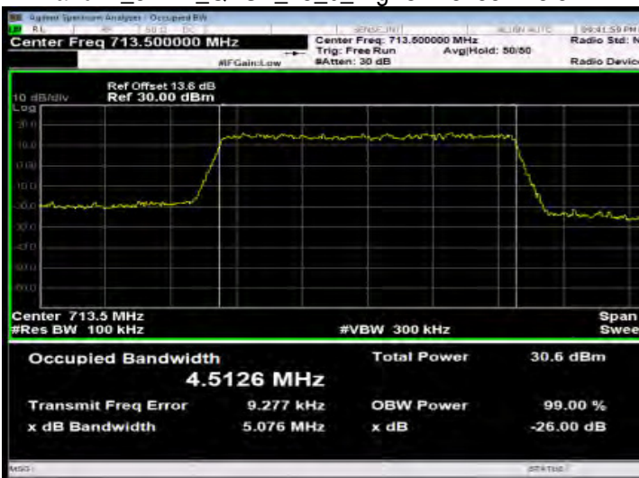
Band12_5MHz_QPSK_25_0_HighCH23155-713.5
