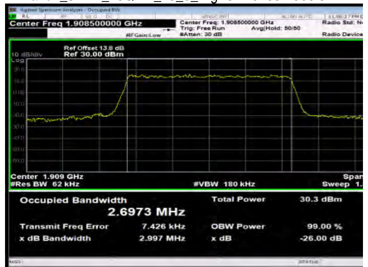
Band2_3MHz_16QAM_15_0_HighCH19185-1908.5
