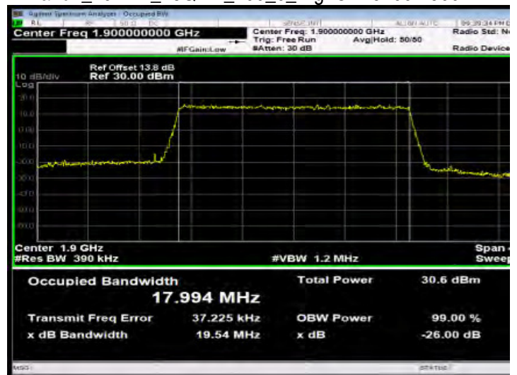
Band2_20MHz_16QAM_100_0_HighCH19100-1900
