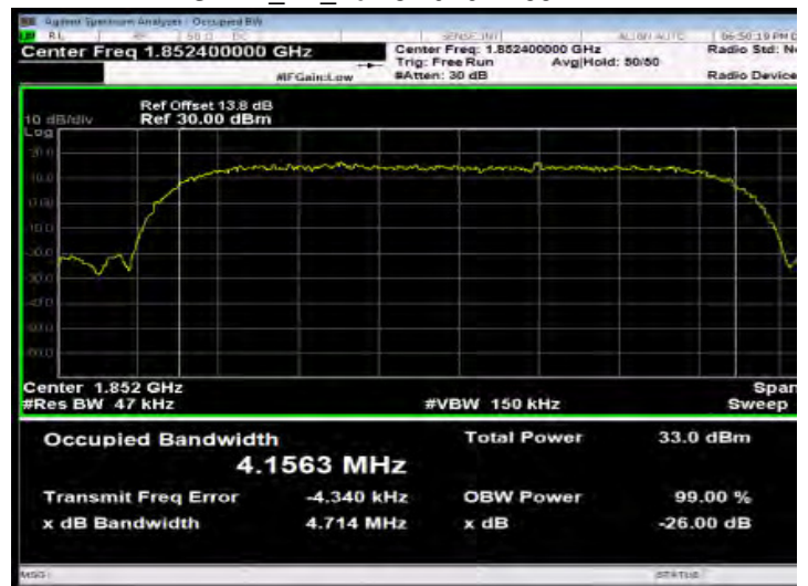
HSDPA_B2_LowCH9262-1852.4
