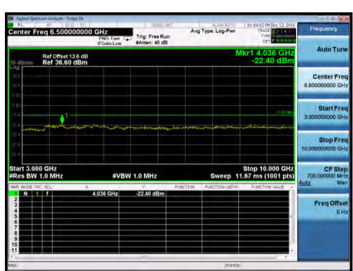
3GHz~10GHz_EDGE_850MHz_MidCH190-836.6
