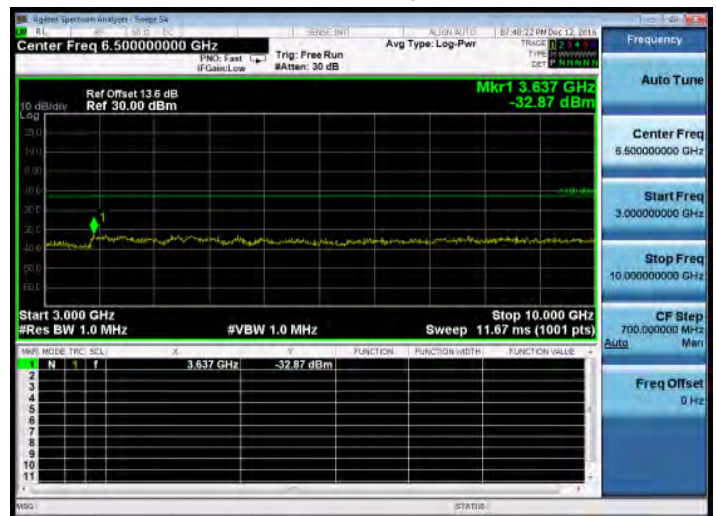
3GHz~10GHz_WCDMA_B5_HighCH4233-846.6
