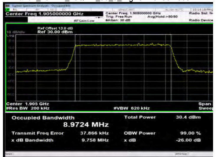
Band2_10MHz_16QAM_50_0_HighCH19150-1905
