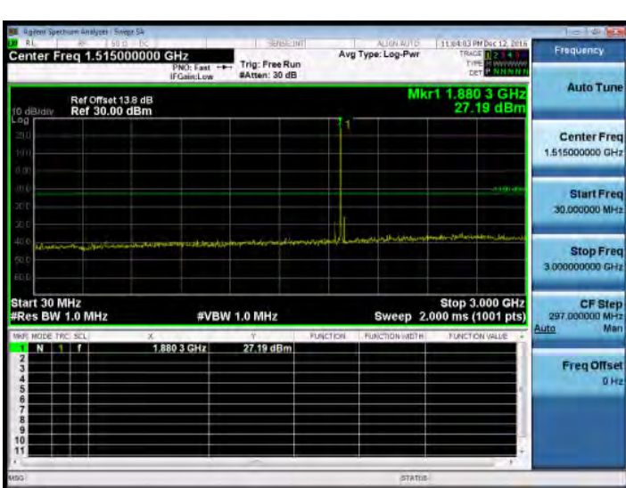
30MHz-3GHz_Band2_1.4MHz_QPSK_1_0_MidCH18900-1880
