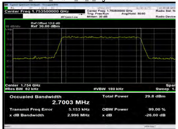
Band4_3MHz_16QAM_15_0_HighCH20385-1753.5
