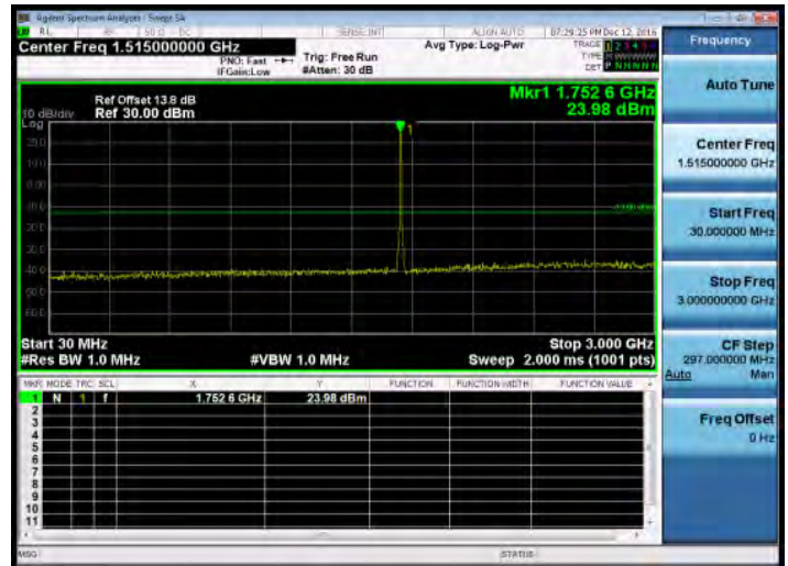
30MHz~3GHz_HSUPA_B4_HighCH1513-1752.6
