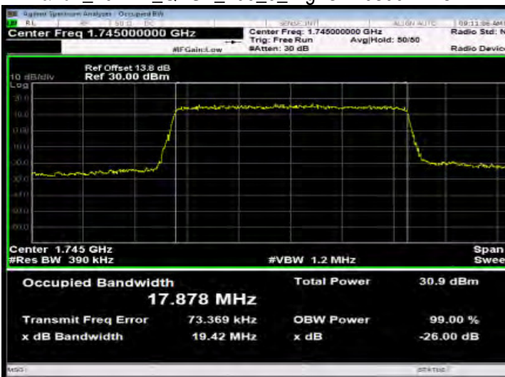
Band4_20MHz_QPSK_100_0_HighCH20300-1745
