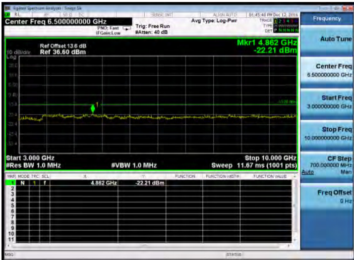
3GHz~10GHz_EDGE_850MHz_HighCH251-848.8
