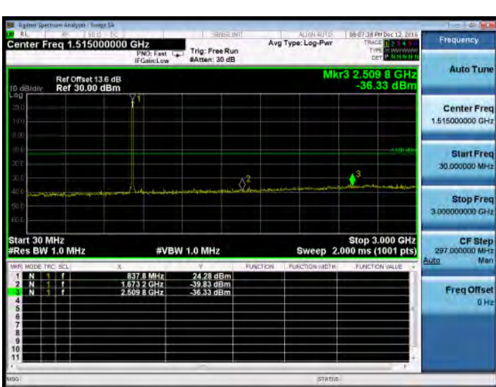
30MHz~3GHz_HSUPA_B5_MidCH4183-836.6
