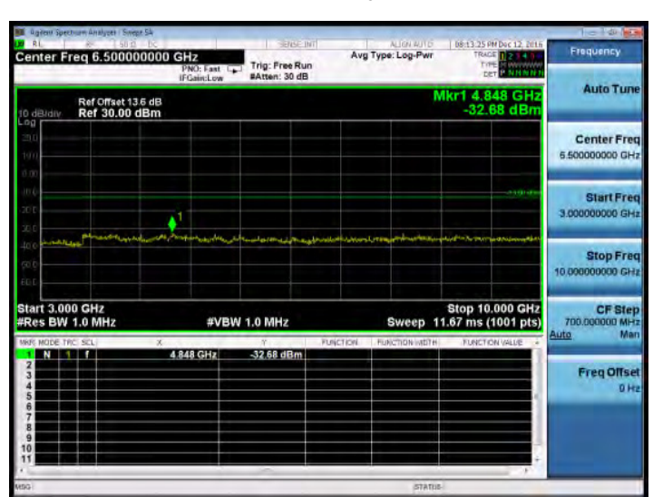
3GHz~10GHz_HSUPA_B5_HighCH4233-846.6
