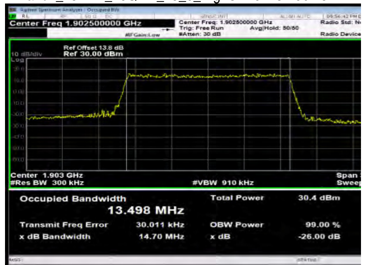
Band2_15MHz_16QAM_75_0_HighCH19125-1902.5
