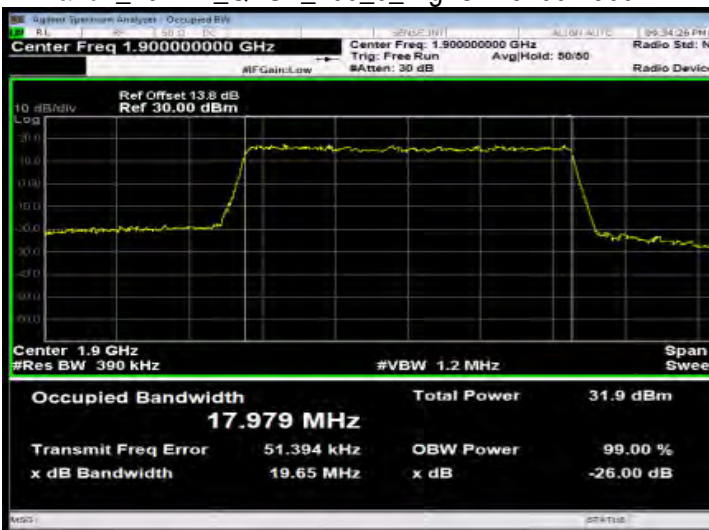
Band2_20MHz_QPSK_100_0_HighCH19100-1900
