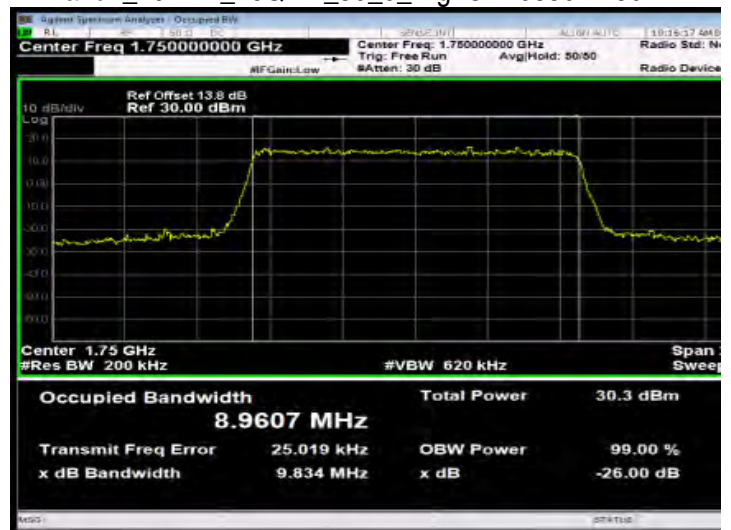
Band4_10MHz_16QAM_50_0_HighCH20350-1750
