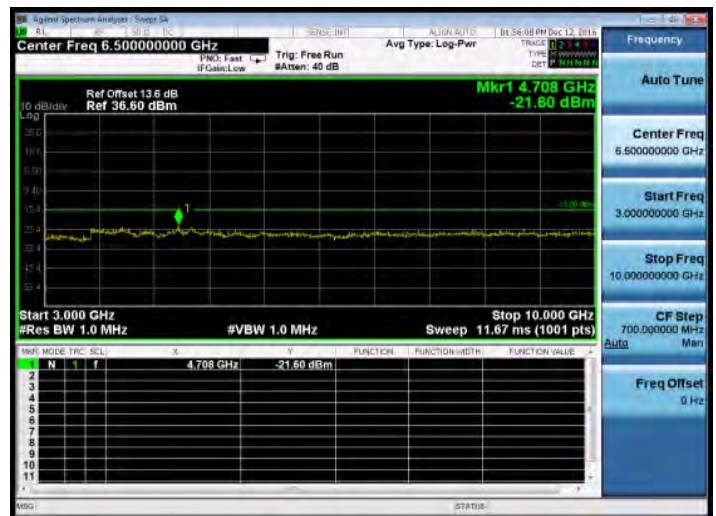
3GHz~10GHz_GPRS_850MHz_MidCH190-836.6
