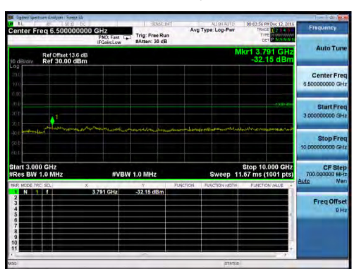
3GHz~10GHz_HSDPA_B5_HighCH4233-846.6
