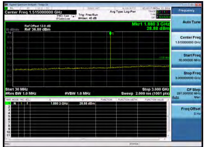
30MHz~3GHz_EDGE_1900MHz_MidCH661-1880
