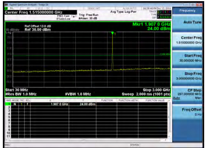
30MHz~3GHz_HSDPA_B2_HighCH9538-1907.6
