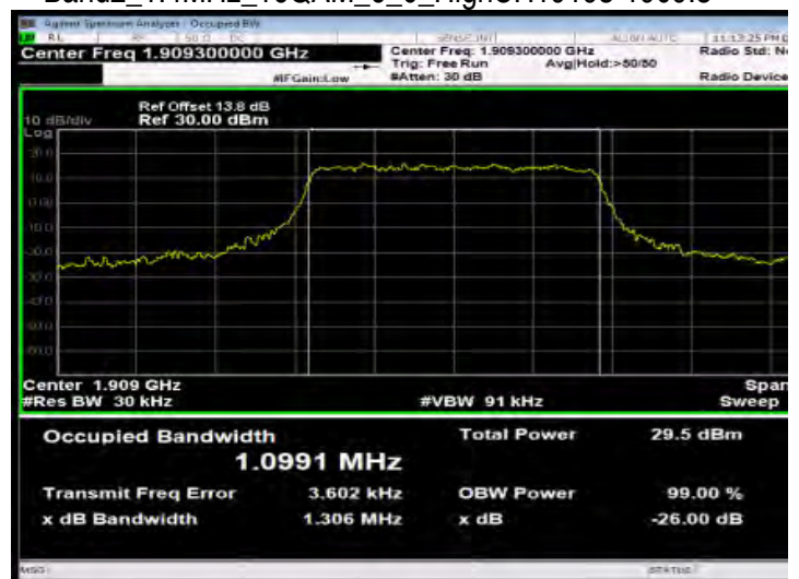
Band2_1.4MHz_16QAM_6_0_HighCH19193-1909.3
