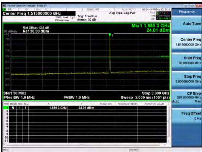
30MHz~3GHz_WCDMA_B2_MidCH9400-1880
