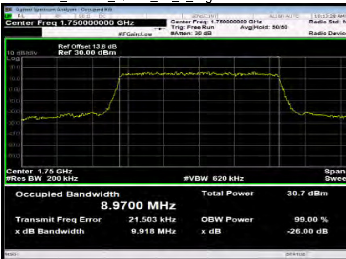
Band4_10MHz_QPSK_50_0_HighCH20350-1750
