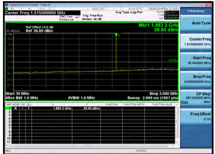
30MHz~3GHz_GSM_1900MHz_MidCH661-1880
