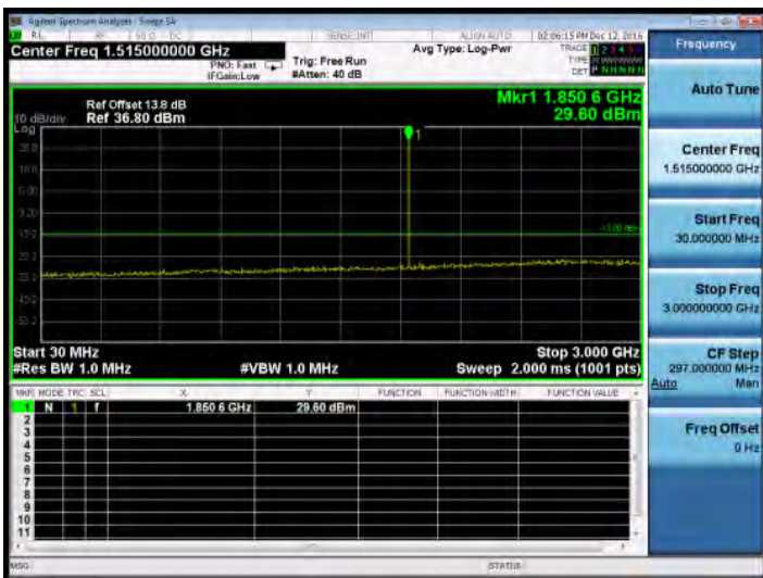
30MHz~3GHz_GSM_1900MHz_LowCH512-1850.2
