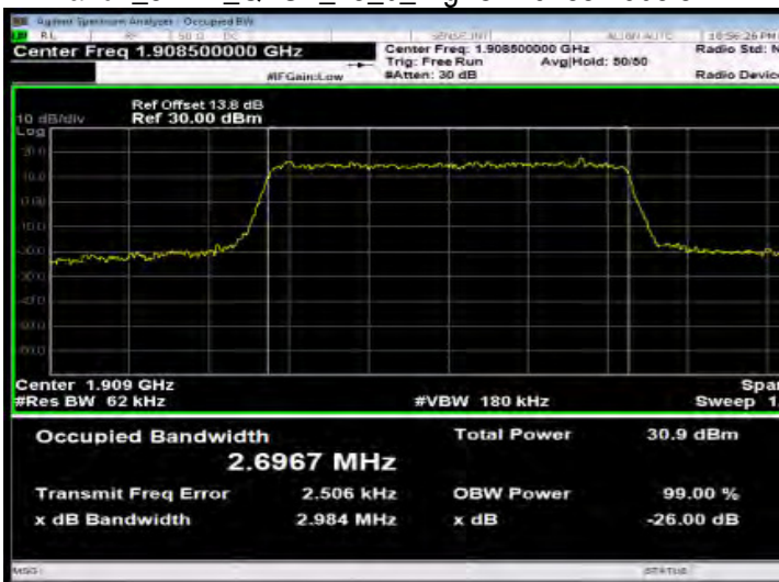
Band2_3MHz_QPSK_15_0_HighCH19185-1908.5
