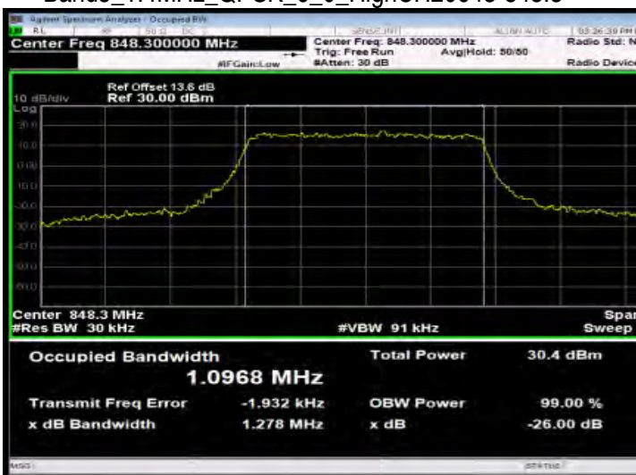
Band5_1.4MHz_QPSK_6_0_HighCH20643-848.3
