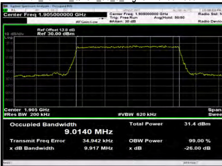
Band2_10MHz_QPSK_50_0_HighCH19150-1905
