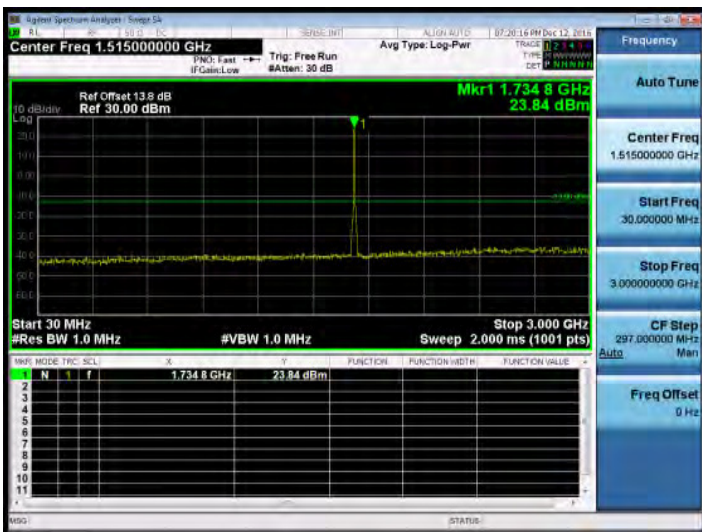
30MHz~3GHz_HSDPA_B4_MidCH1413-1732.6
