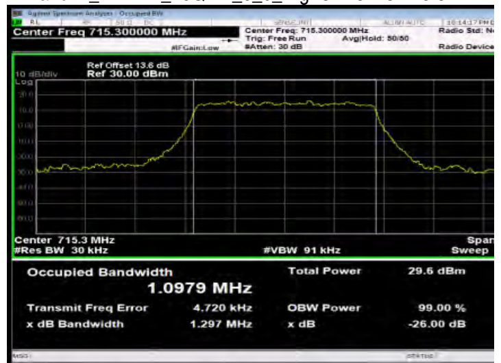
Band12_1.4MHz_16QAM_6_0_HighCH23173-715.3
