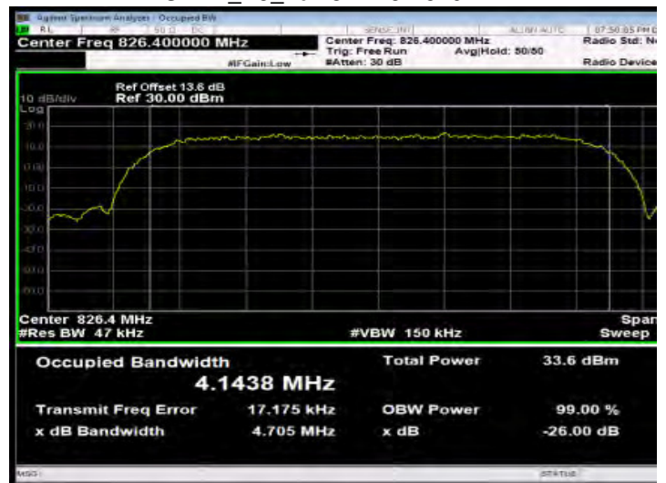
HSDPA_B5_LowCH4132-826.4
