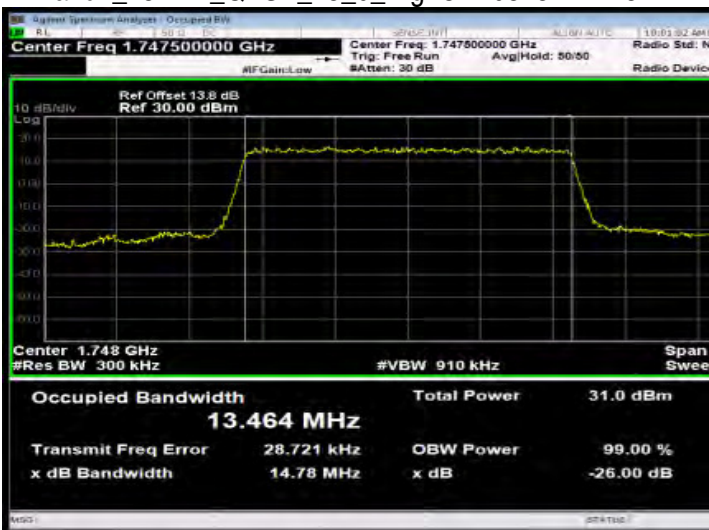
Band4_15MHz_QPSK_75_0_HighCH20325-1747.5
