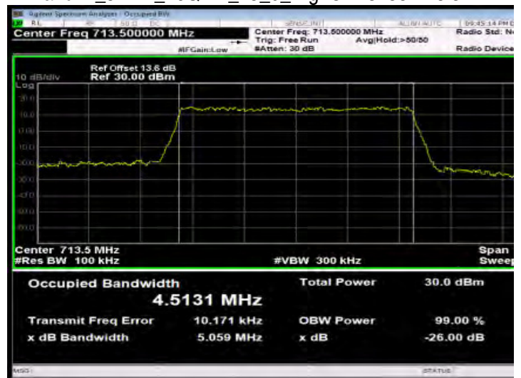
Band12_5MHz_16QAM_25_0_HighCH23155-713.5
