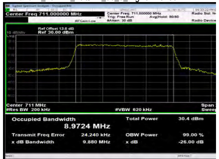
Band12_10MHz_16QAM_50_0_HighCH23130-711
