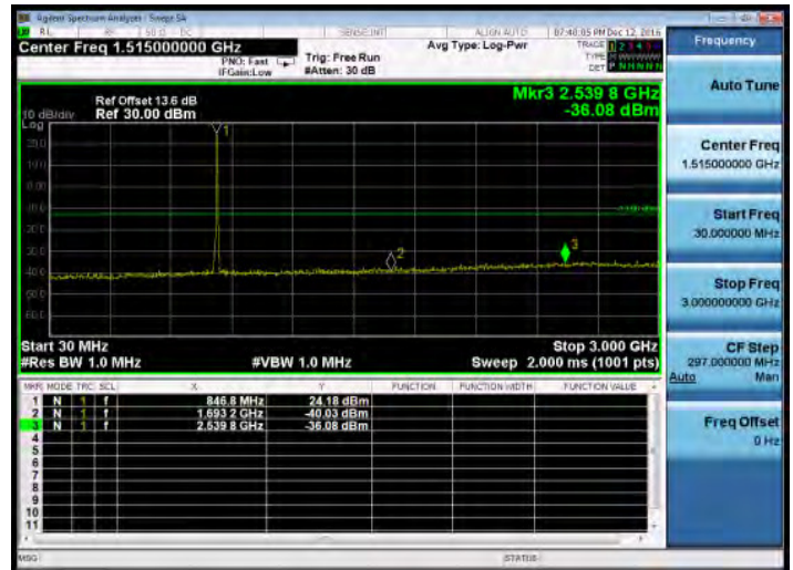
30MHz~3GHz_WCDMA_B5_HighCH4233-846.6
