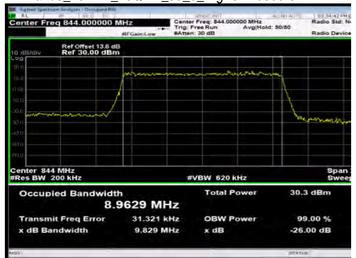
Band5_10MHz_16QAM_50_0_HighCH20600-844
