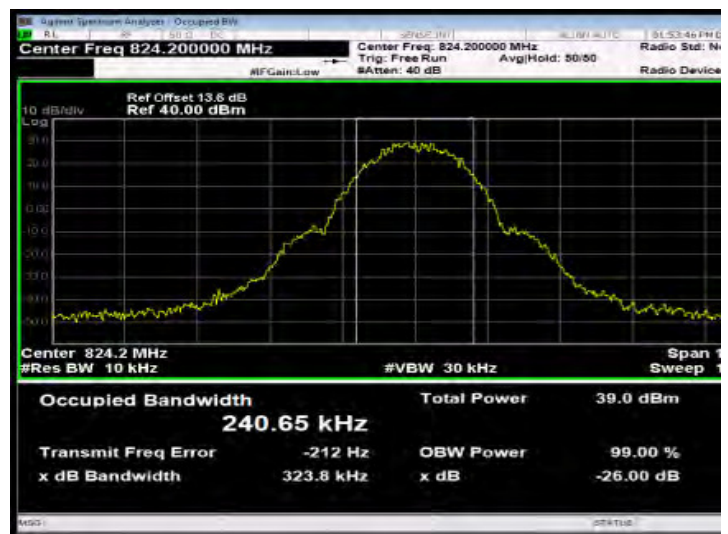
GPRS_850MHz_LowCH128-824.2
