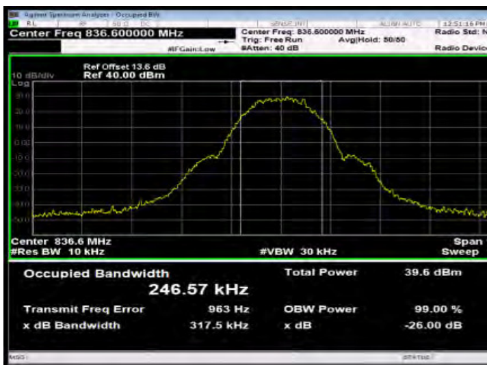
GSM_850MHz_MidCH190-836.6
