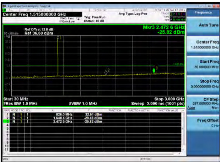
30MHz~3GHz_GPRS_850MHz_LowCH128-824.2
