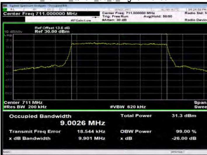
Band12_10MHz_QPSK_50_0_HighCH23130-711
