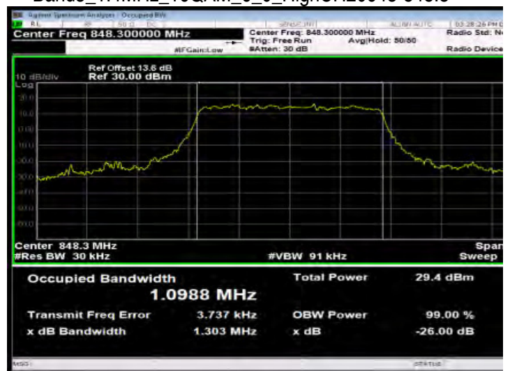
Band5_1.4MHz_16QAM_6_0_HighCH20643-848.3
