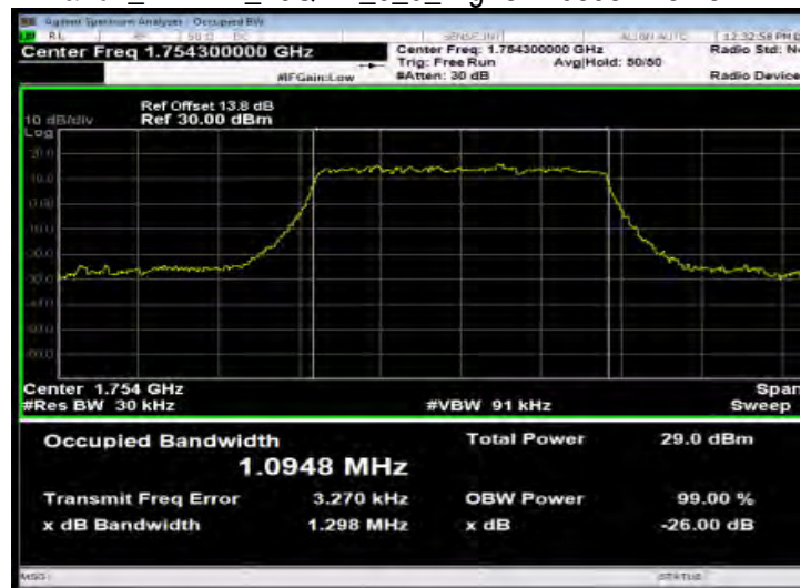
Band4_1.4MHz_16QAM_6_0_HighCH20393-1754.3
