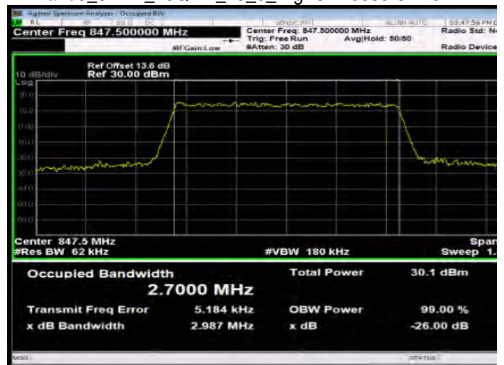
Band5_3MHz_16QAM_15_0_HighCH20635-847.5
