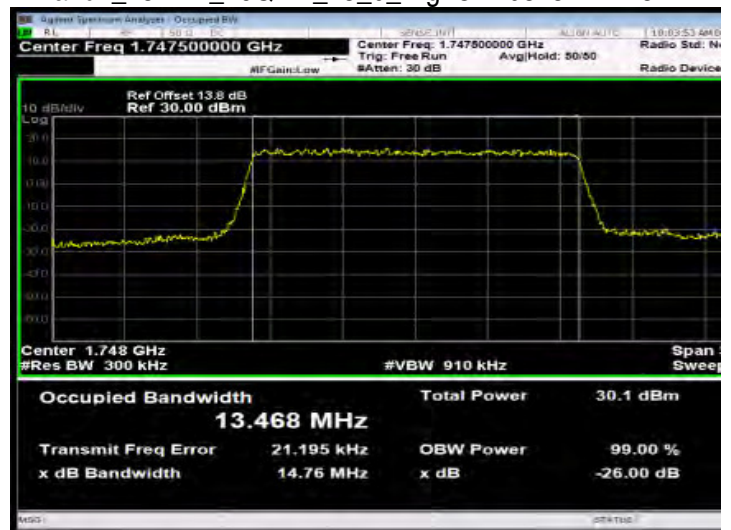
Band4_15MHz_16QAM_75_0_HighCH20325-1747.5
