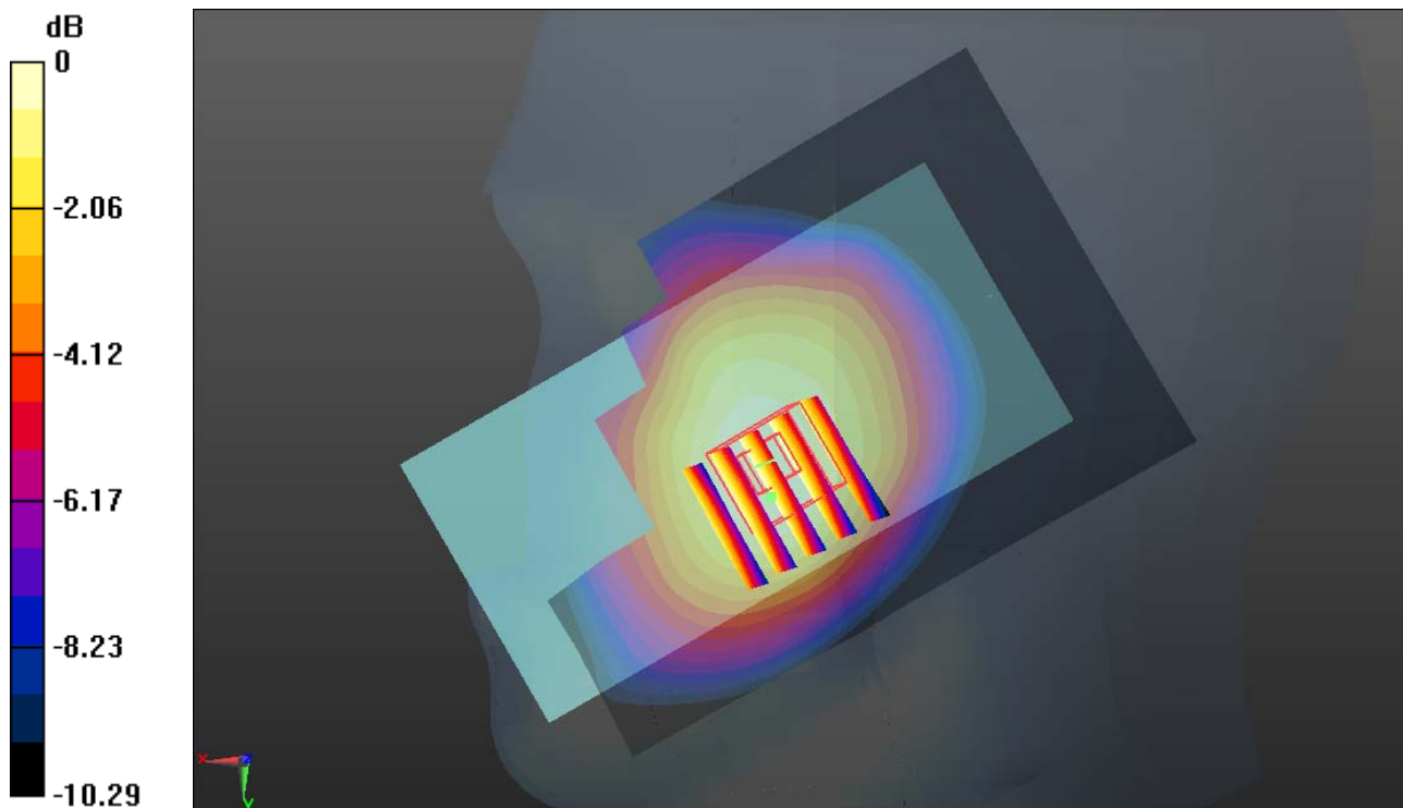
0 dB = 0.380mW/g
