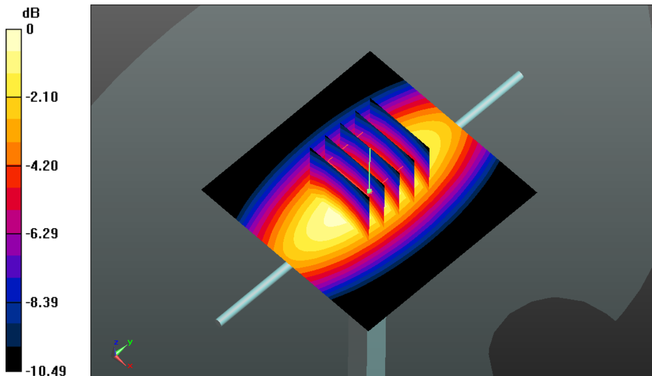
0 dB = 2.870\text{mW/g}
