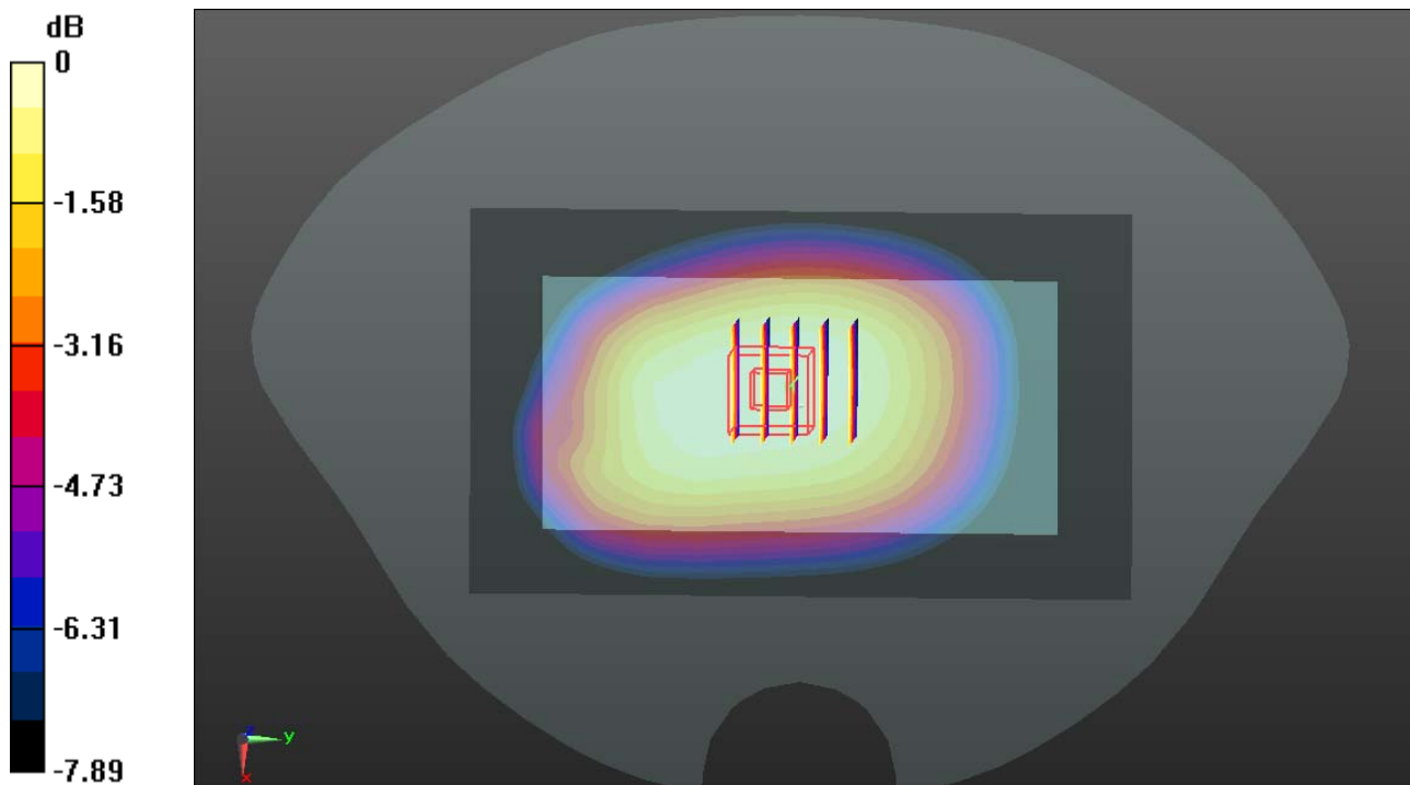
0 dB = 0.570mW/g
