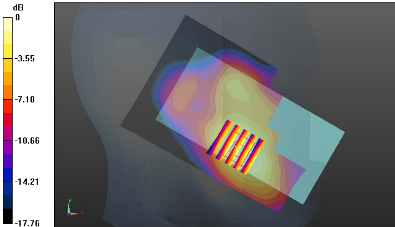
0 dB = 0.470\text{mW/g}
