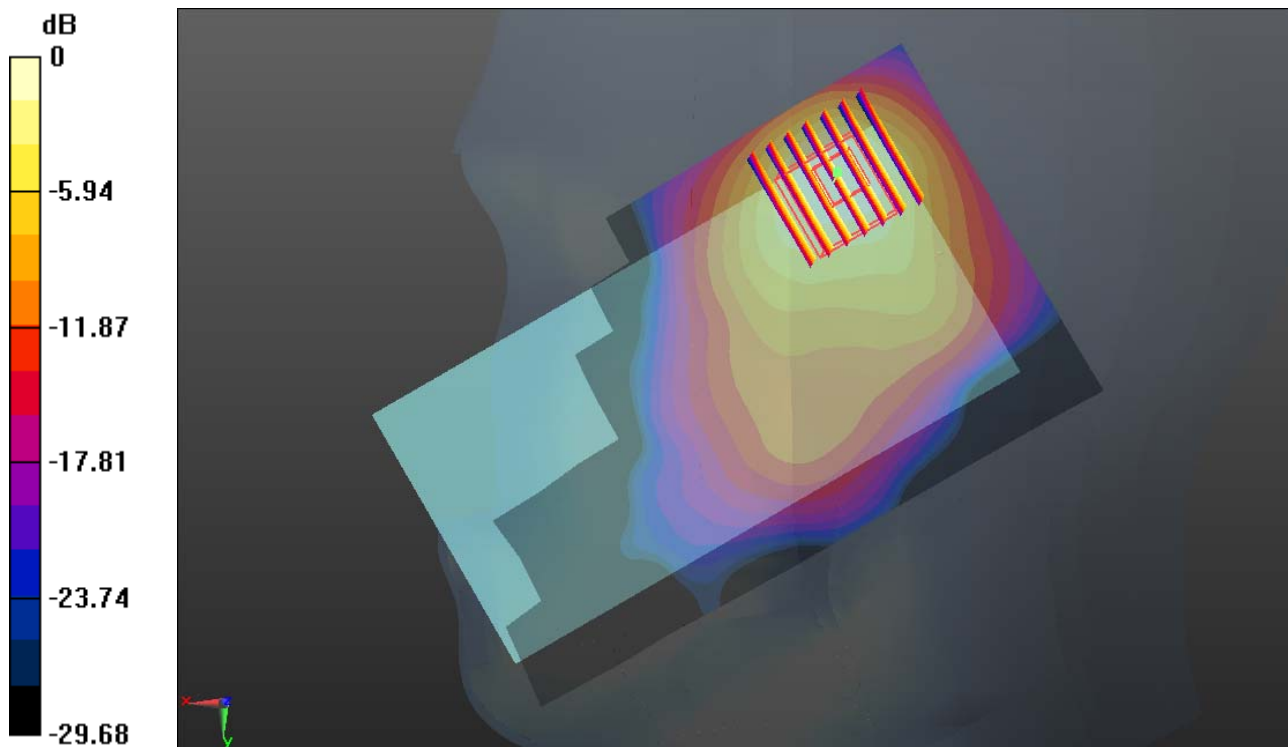
0 dB = 1.290mW/g
