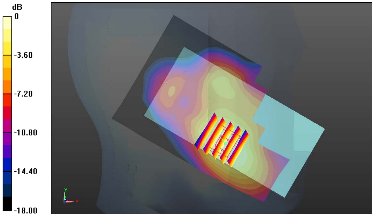
0 dB = 0.360mW/g
