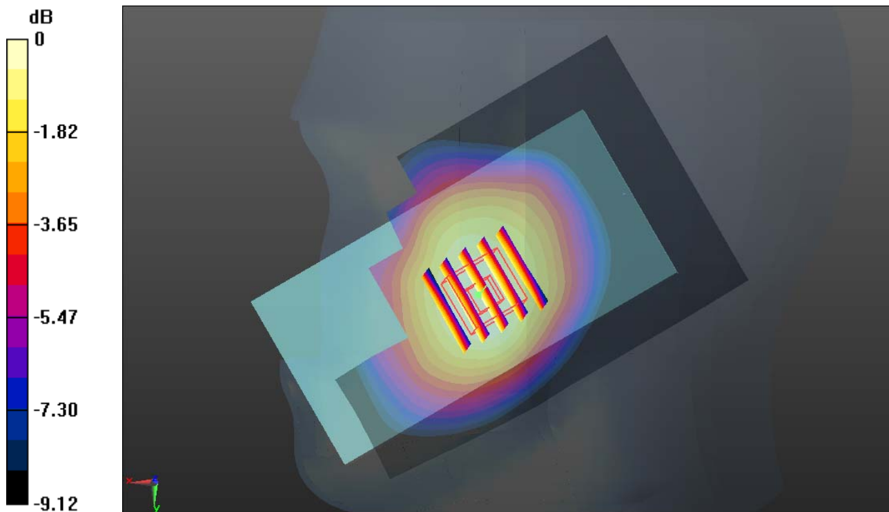
0 dB = 0.960mW/g
