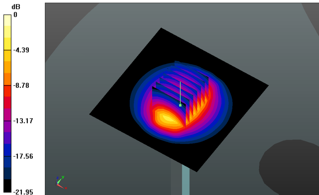
0 dB = 19.600mW/g
