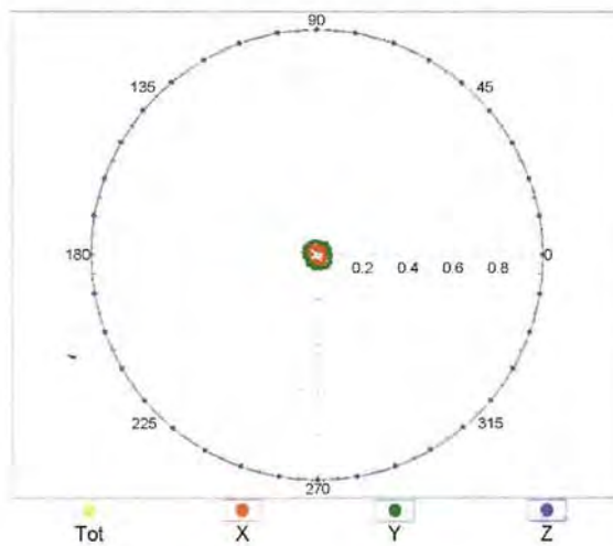
f=600 MHz,TEM,90°
