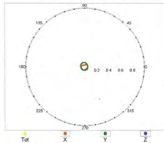
f=2500 MHz,R22,90°
