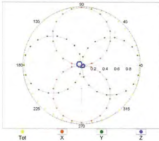
f=600 MHz,TEM,0°
