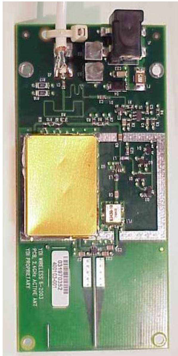
Photograph of EUT – Internal View Component side
