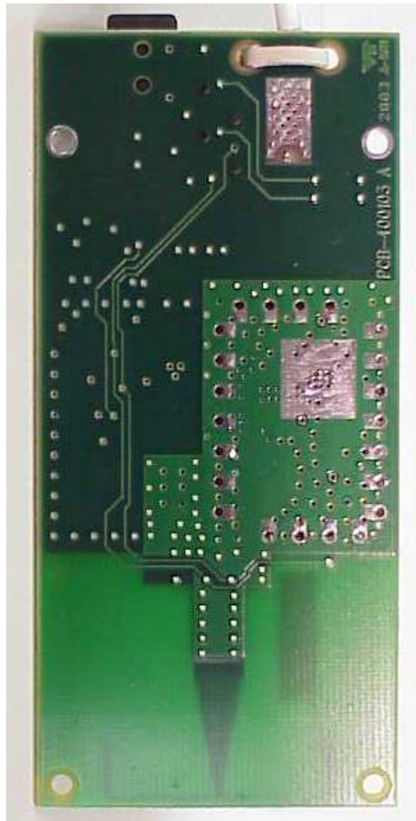
Photograph of EUT – Internal View Copper side
