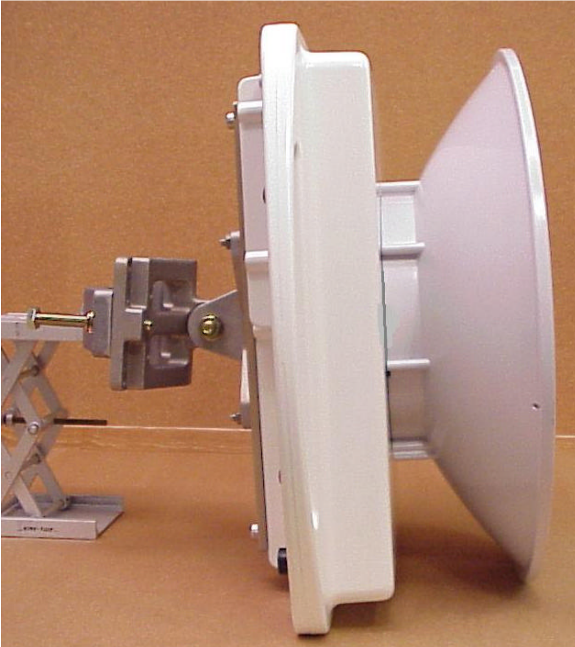
Photograph of EUT – side view
