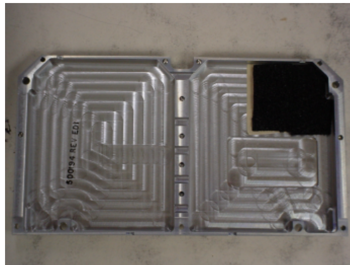
Bottom view of 24GHz RF module shield
