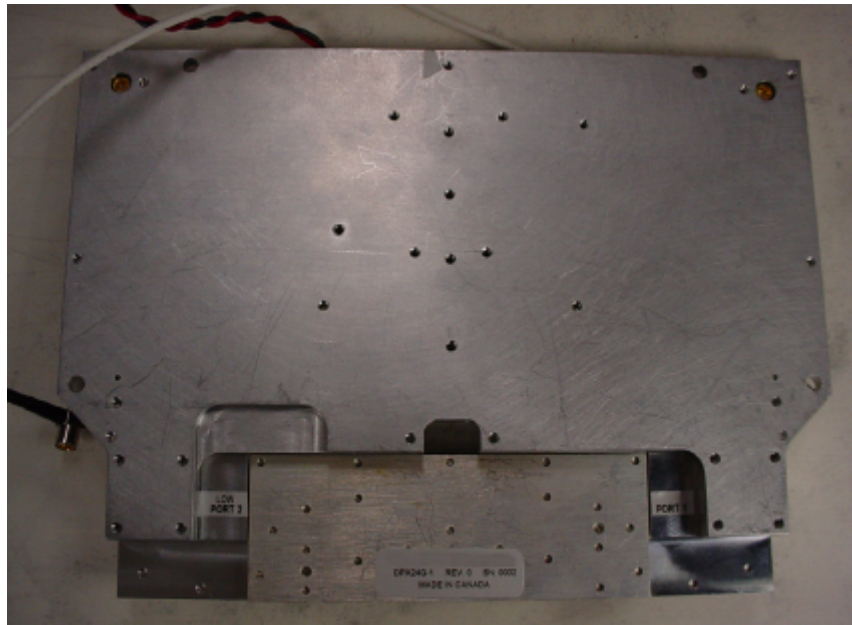
Bottom view of 24GHz RF module with attached duplexer
