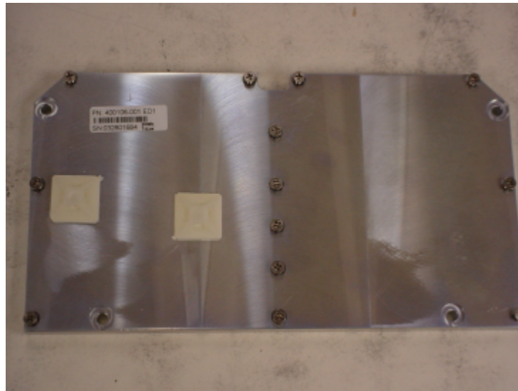
Top view of 24GHz RF module shield
