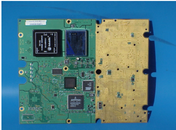
Link CX 24GHz PCB bottom view without shields
