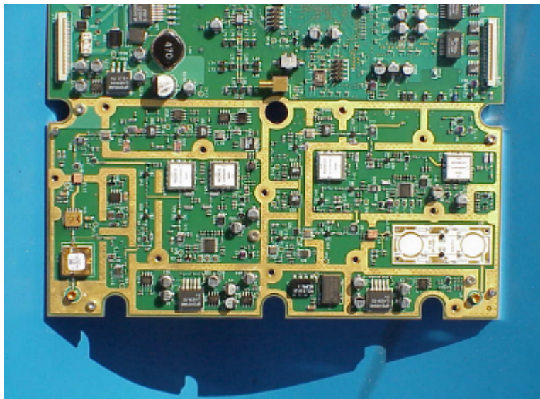
Link CX 24GHz PCB top view, RF section close-up
