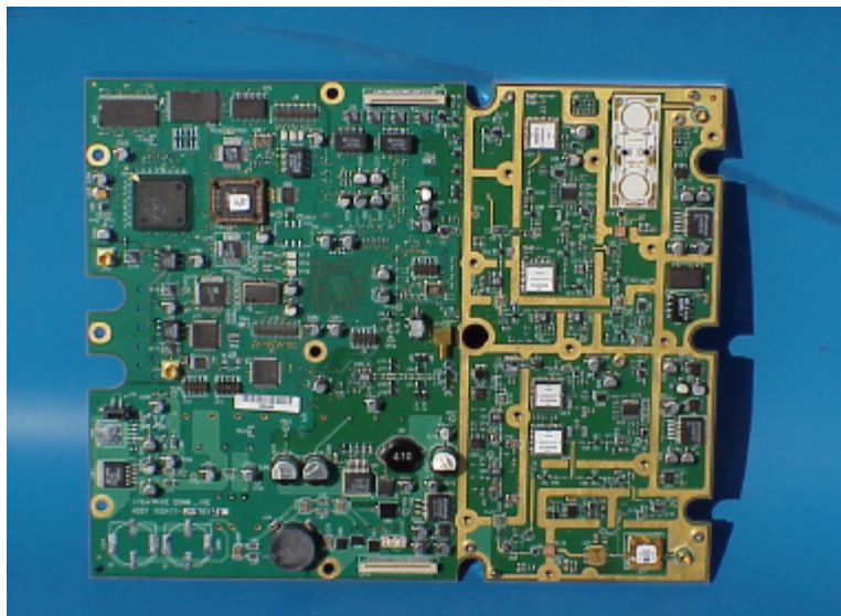
Link CX 24GHz PCB top view without shields
