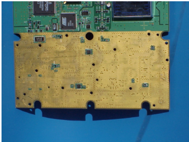
Link CX 24GHz PCB bottom view, RF section close-up
