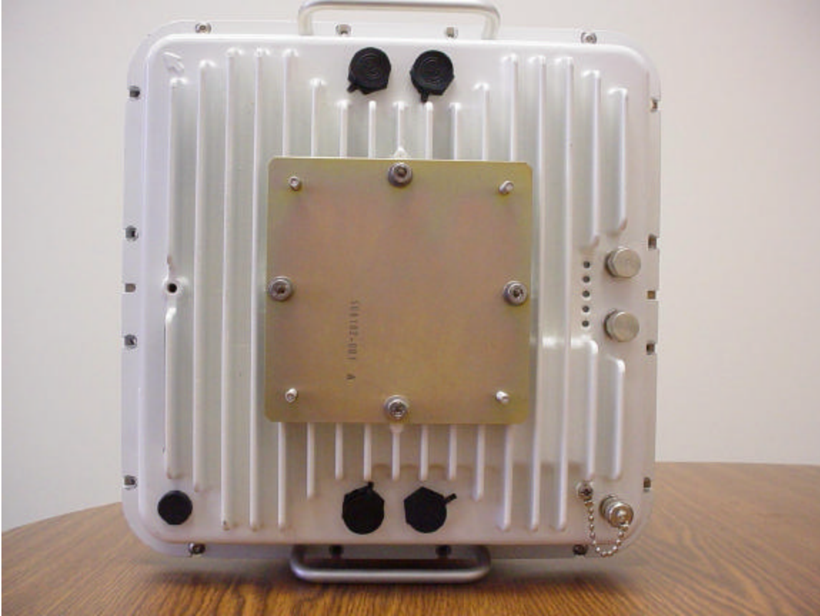
Photograph of EUT – rear view
