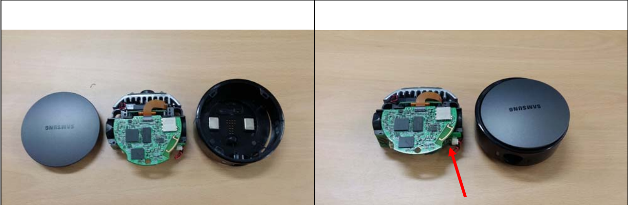
WIFI Antenna
