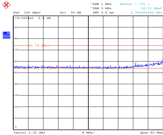
Lowest Channel(2 422 Mhz): Peak
