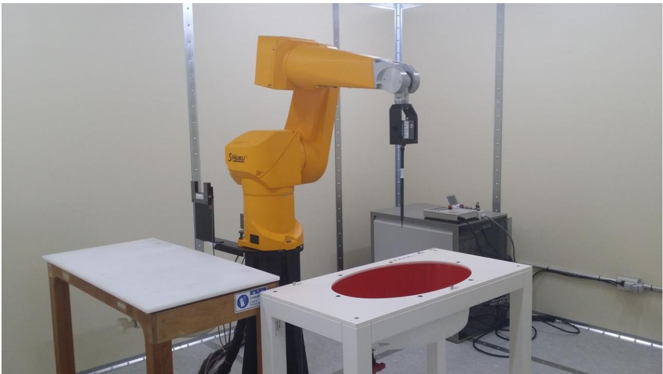
Figure 3. SPEAG DASY 4
