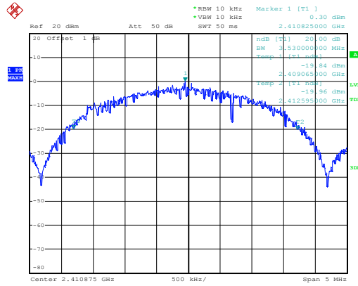
Figure 5. Plot of the 20dB Channel Bandwidth (Conducted)
