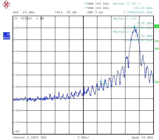
Figure 10. Plot of the Band Edge (Conducted)
