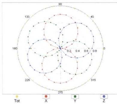
f=600 MHz,TEM
