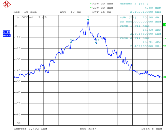
Figure 5. Plot of the 20dB Channel Bandwidth (Conducted)
