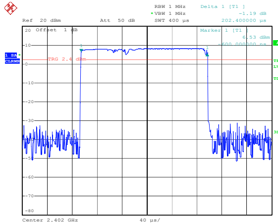
Figure 8. Plot of the Time of Occupancy (Conducted)
