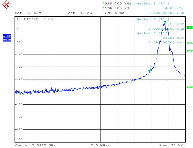
Figure 10. Plot of the Band Edge (Conducted)
