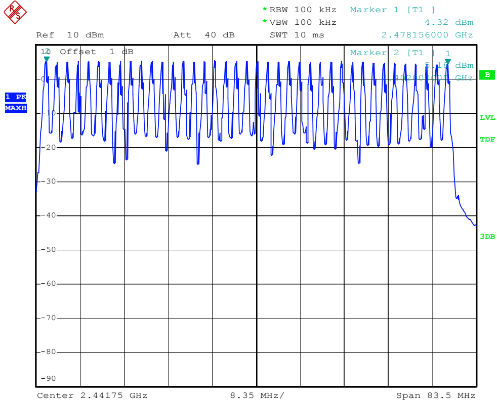
Figure 7. Plot of the Number of Hopping Channels (Conducted)
