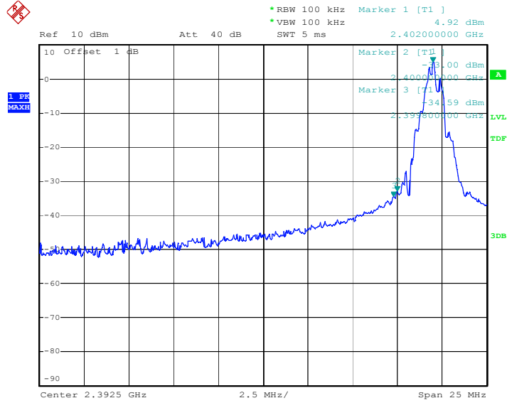
Figure 10. Plot of the Band Edge (Conducted)
