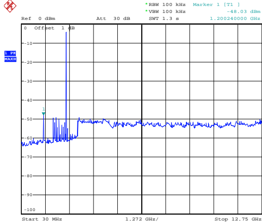
Figure 12. Plot of the Spurious RF conducted emissions
