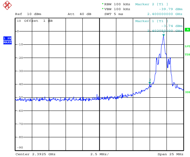
Figure 10. Plot of the Band Edge (Conducted)
