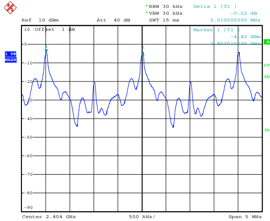
Figure 3. Plot of the Carrier Frequency Separation (Conducted)
