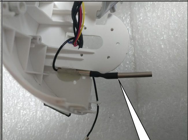
Wi-Fi Antenna
