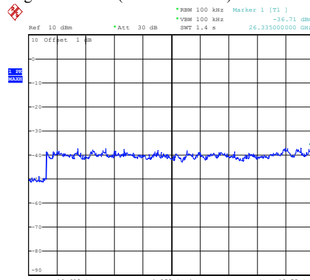
Highest Channel(2471.625 MHz):12.75~26.5GHz
