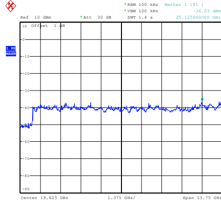
Lowest Channel(2410.875 MHz):12.75~26.5GHz
