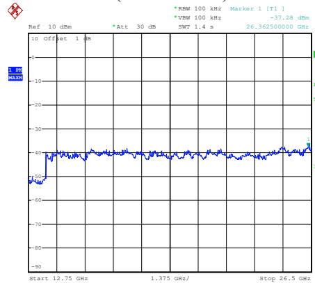
Middle Channel(2441.250 MHz):12.75~26.5GHz
