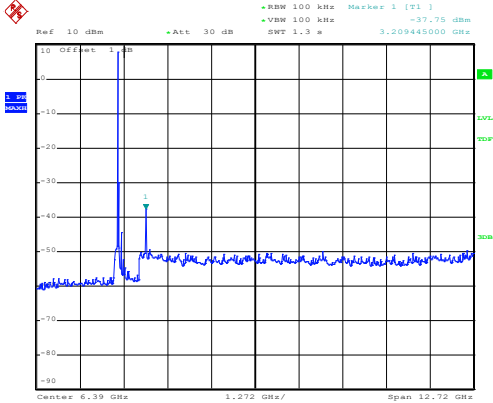
Lowest Channel(2 410.875 MHz):30MHz~12.75GHz
