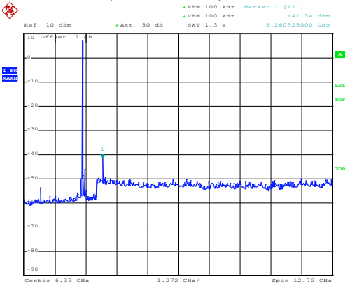
Middle Channel(2 441.250 MHz):30MHz~12.75GHz
