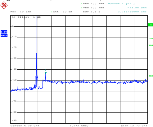
Highest Channel(2 471.625 MHz):30MHz~12.75GHz
