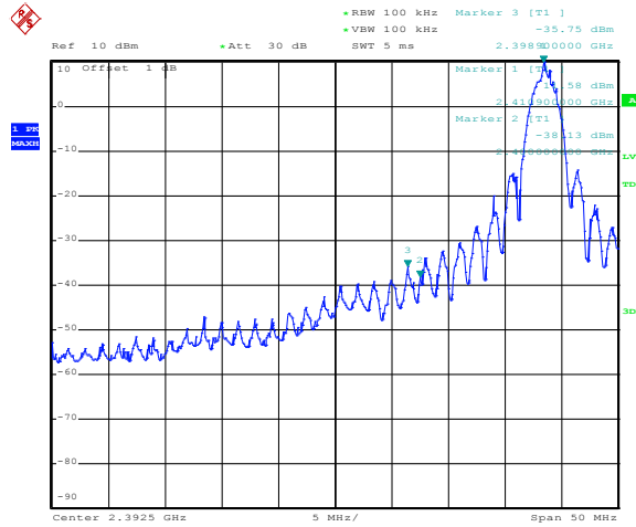
Figure 10. Plot of the Band Edge (Conducted)
