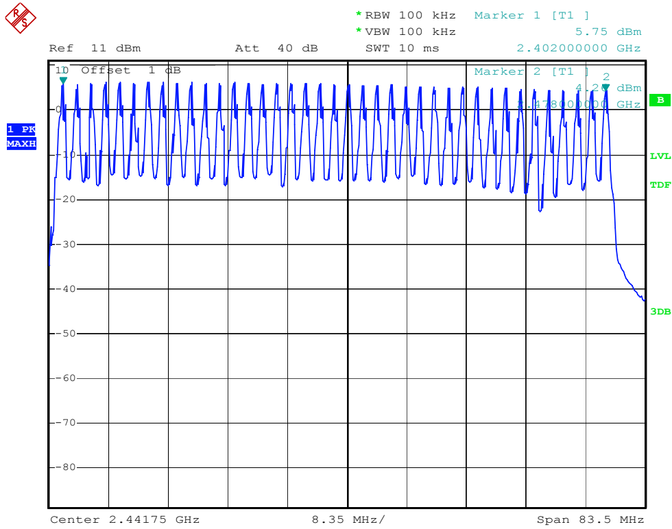
Figure 7. Plot of the Number of Hopping Channels (Conducted)
