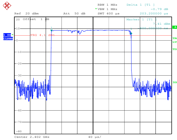
Figure 8. Plot of the Time of Occupancy (Conducted)
