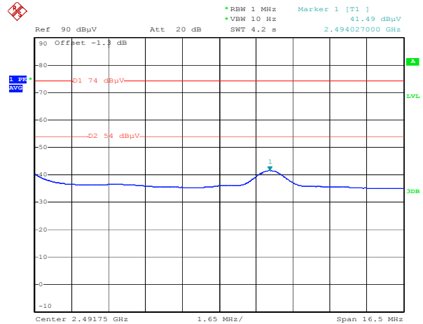
Highest Channel(2478 MHz): AVERAGE
