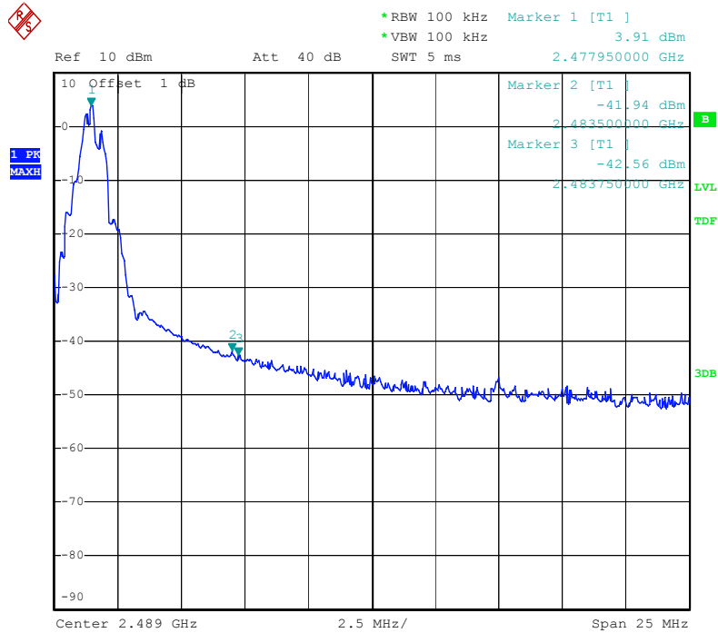
Highest Channel (2478 MHz)
