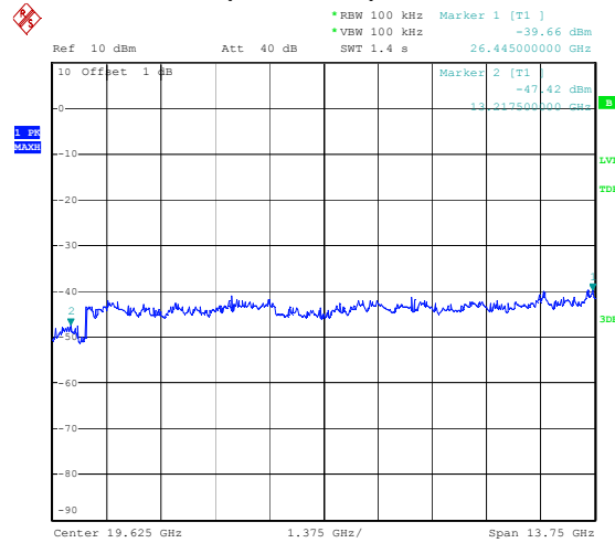
Figure 12. Plot of the Spurious RF conducted emissions
