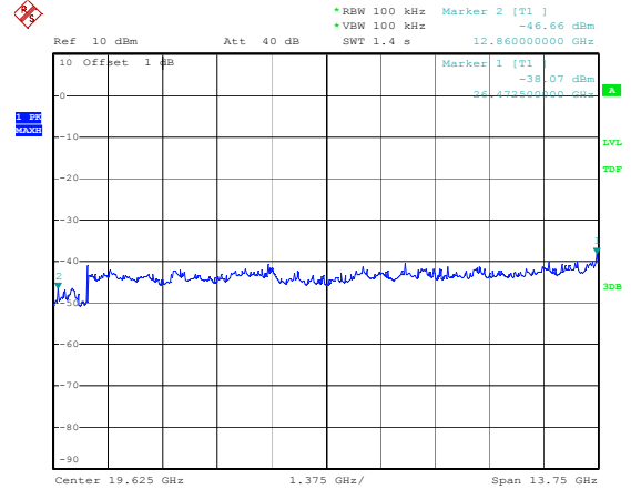
Highest Channel(2478 MHz):12.75~26.5GHz
