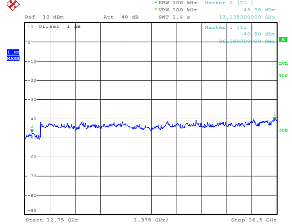
Middle Channel(2440 MHz):12.75~26.5GHz
