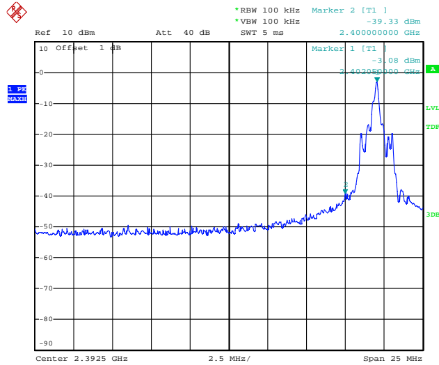
Figure 10. Plot of the Band Edge (Conducted)
