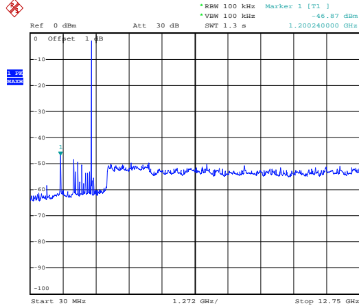
Middle Channel(2440 MHz):30MHz~12.75GHz
