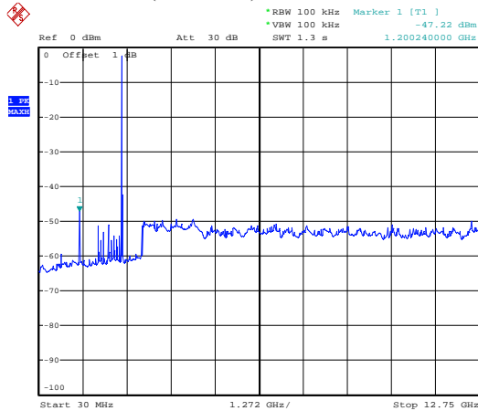
Highest Channel(2480 MHz):30MHz~12.75GHz
