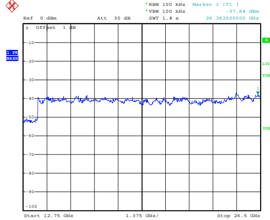
Middle Channel(2440 MHz):12.75~26.5GHz
