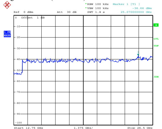
Highest Channel(2480 MHz):12.75~26.5GHz
