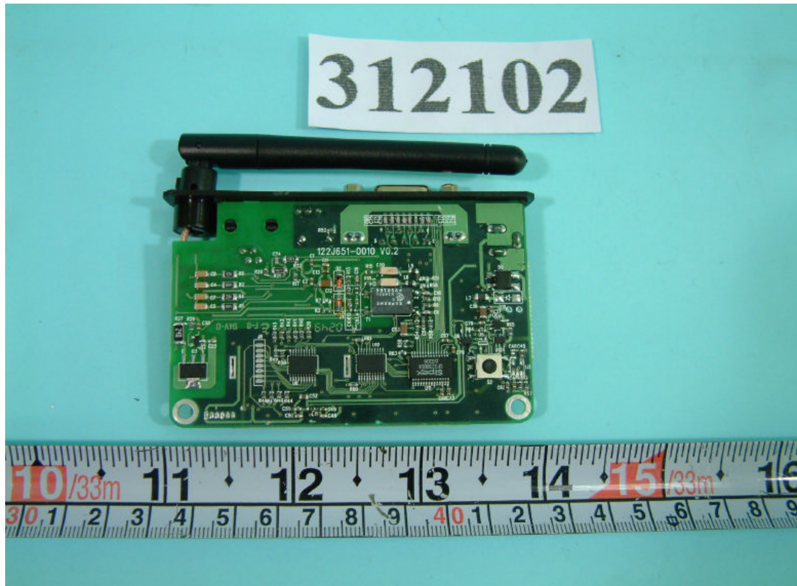
Rear side of Main Board
