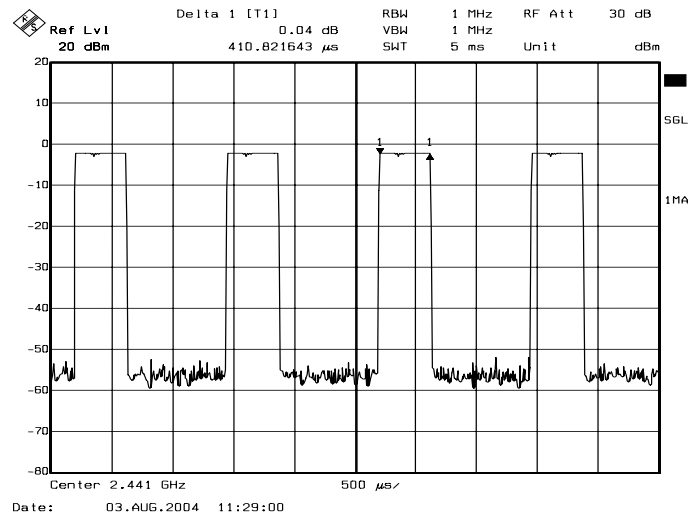
DH1 2441MHz
