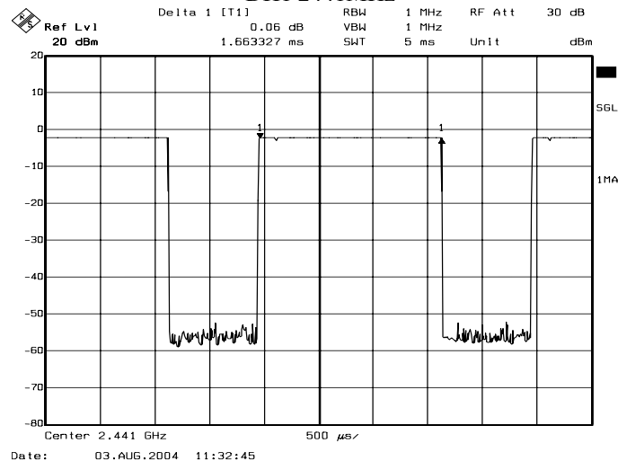
DH3 2441MHz
