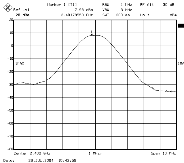
Channel Low
