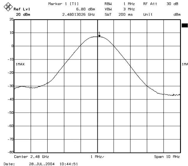
Channel High
