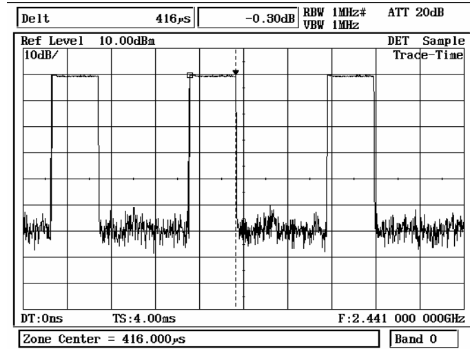
DH1 2441MHz
