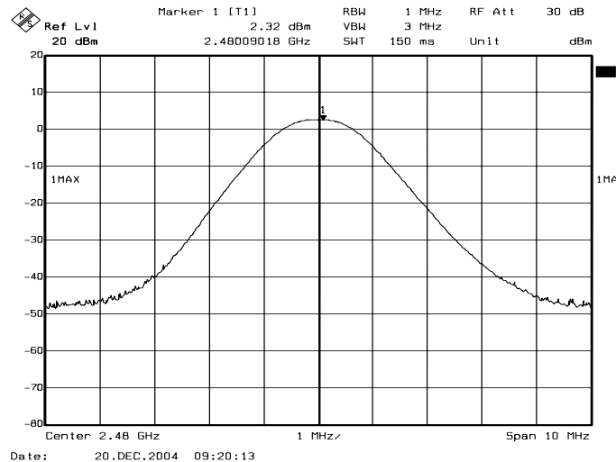
Channel High
