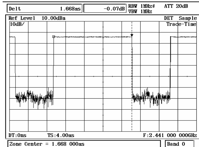
DH3 2441MHz
