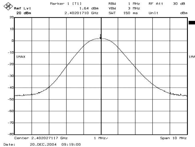
Channel Low
