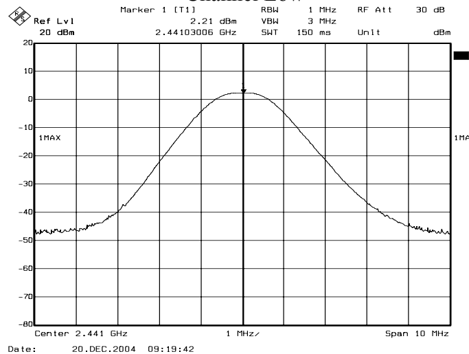
Channel Middle
