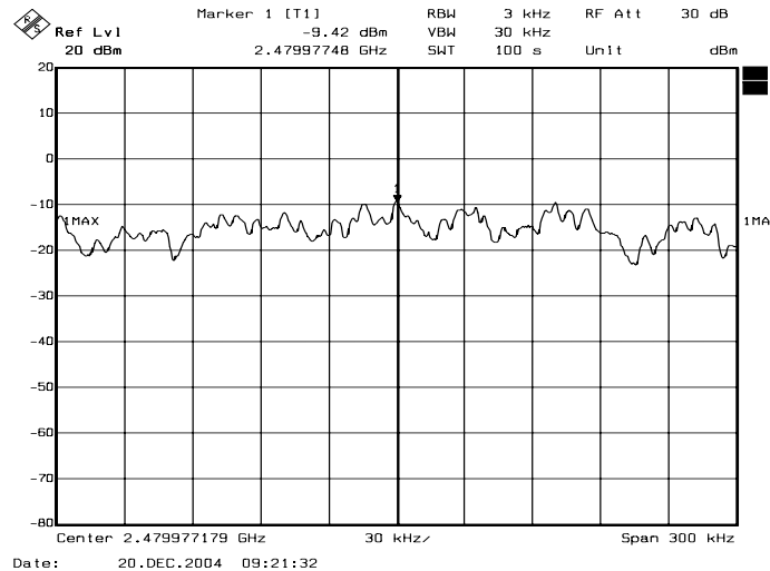
Channel High
