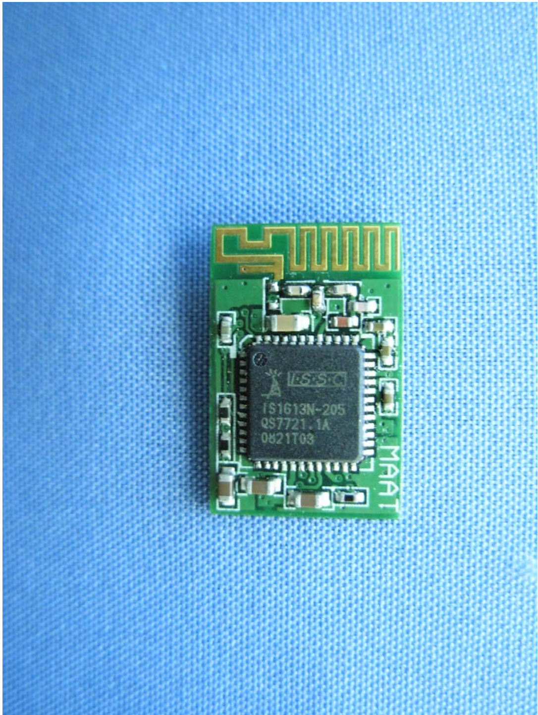
(7) EUT Photo
